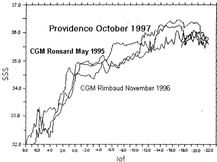
Fig. 5 - SSS intensive observation by thermosalinograph on the commercial line Panama-Tahiti.
