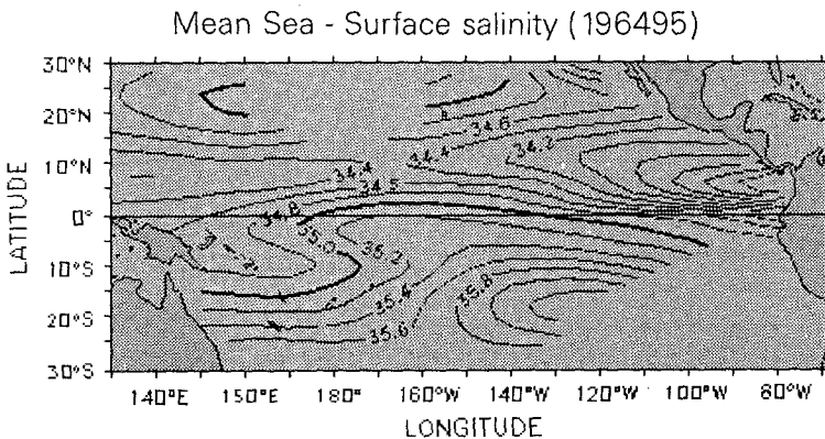
Fig. 1 - Basin-wide mean sea surface salinity over the 1964-1995 period.
