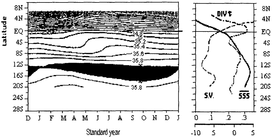
Fig. 3 - Variations along the track Tahiti-Panama of: (left): Seasonal SSS cycle; (right): SSS mean, SSS seasonal variability, wind divergence.
