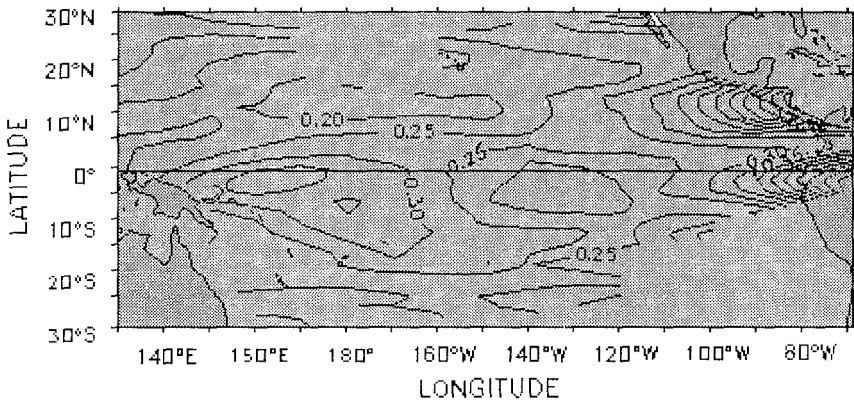
Fig. 2 - Basin-wide sea surface salinity standard deviation over the 1964-1995 period.
