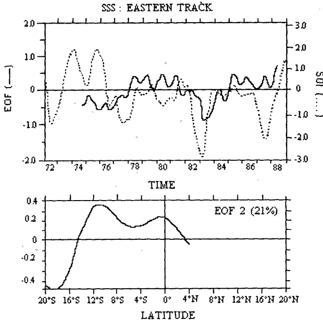
Fig. 4 - Second EOF function of SSS variation. (Top): time function and Southern Oscillation Index; (Bottom): latitudinal distribution along Tahiti-Panama track.
