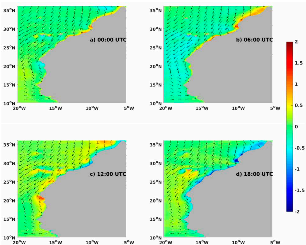
Figure 10. Diurnal 10 m wind speed anomaly (shaded, \text{m s}^{-1} ) estimated as the difference between the seasonal mean for a given synoptic time and the seasonal mean for all synoptic times for January, and the seasonal mean wind velocity for each synoptic time. Results are based on the IFREMER wind analysis, seasonal means are computed over 2000–2018.
