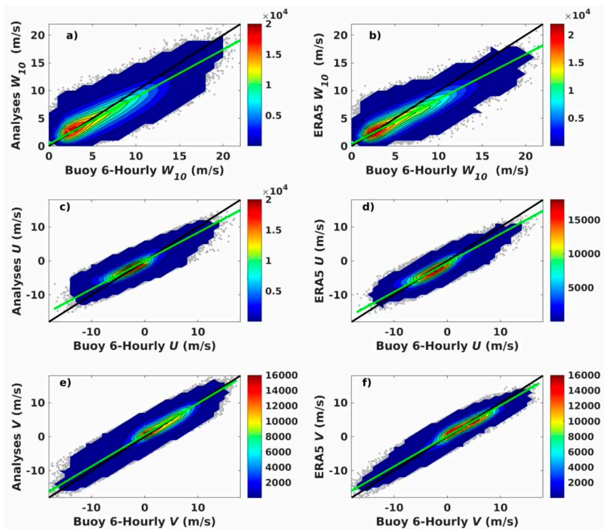
Figure 5. As Figure 4 but for nearshore comparisons.
