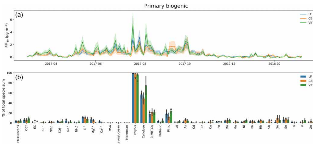
Figure 5. Primary biogenic factor for the three urban sites. (a) Contribution to PM 10 given the mean and standard deviation of the 100 BS. (b) Percentage (%) of each species apportioned by this factor (dots refer to the constrained run, bar plots refer to the mean, and error bars refer to the standard deviation of the 100 BS).
