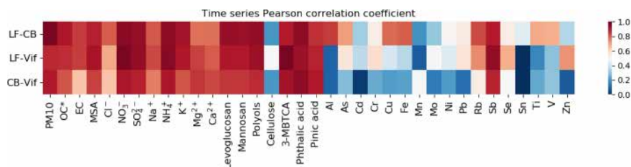
Figure 3. Concentration time series Pearson correlation coefficient of PM 10 and its chemical composition between LF and CB (LF-CB), LF and Vif (LF-Vif), and CB and Vif (CB-Vif).
