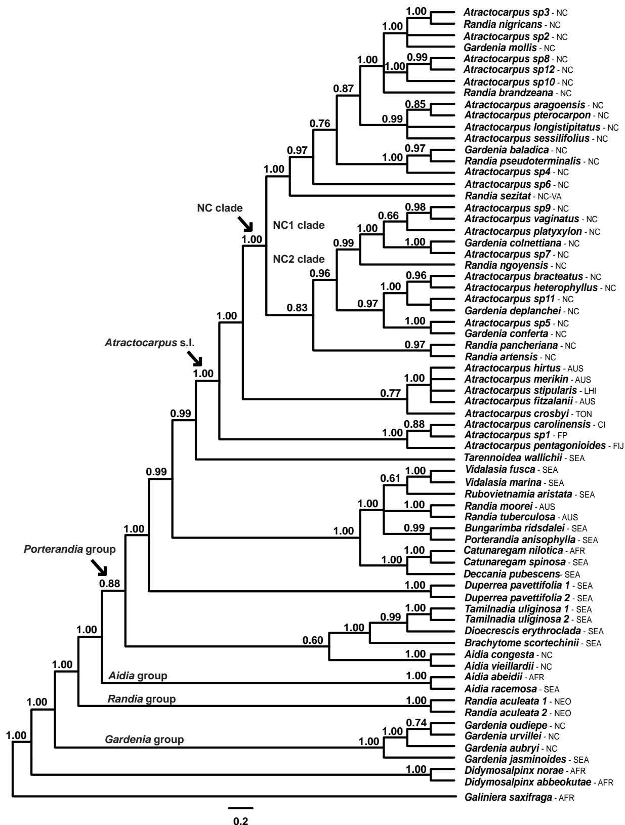
Figure 2 – Phylogenetic tree of the Porterandia group obtained from the combined analysis of cpDNA ( trnTF and rpl32 ) and nrDNA (ITS). Numbers indicate Bayesian posterior probabilities. Areas of distribution are indicated after species names: AFR = Africa; AUS = Australia; CI = Caroline Islands; FIJ = Fiji; FP = French Polynesia; LHI = Lord Howe Islands; NEO = Neotropics; NC = New Caledonia; SEA = South-East Asia; TON = Tonga; VA = Vanuatu.
