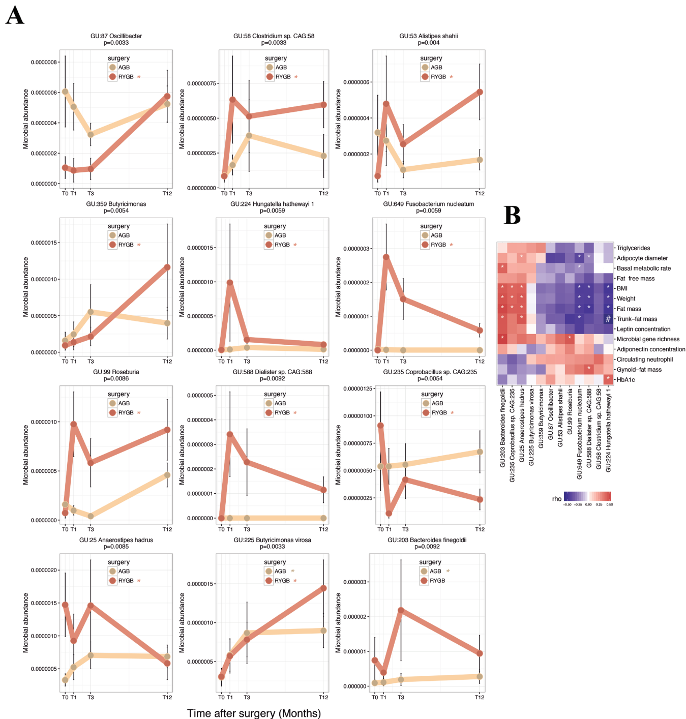
Figure 5 Significant MGS change postbariatric surgery. (A) 12 MGS significantly differ between baseline and T12 post both surgeries. Brown: RYGB (11 MGS); beige: AGB (2 MGS; 1 is common to RYGB-MGS). *Significant p value (in brown for RYGB and beige for AGB between T0 and T12). (B) Heatmap of Spearman's pairwise correlation coefficients between MGS delta and improvement in clinical outcomes. *Significant p value; #significant FDR. AGB, adjustable gastric banding; BMI, body mass index; HbA1c, haemoglobin A1c; MGS, metagenomic species; RYGB, Roux-en-Y-gastric bypass.
