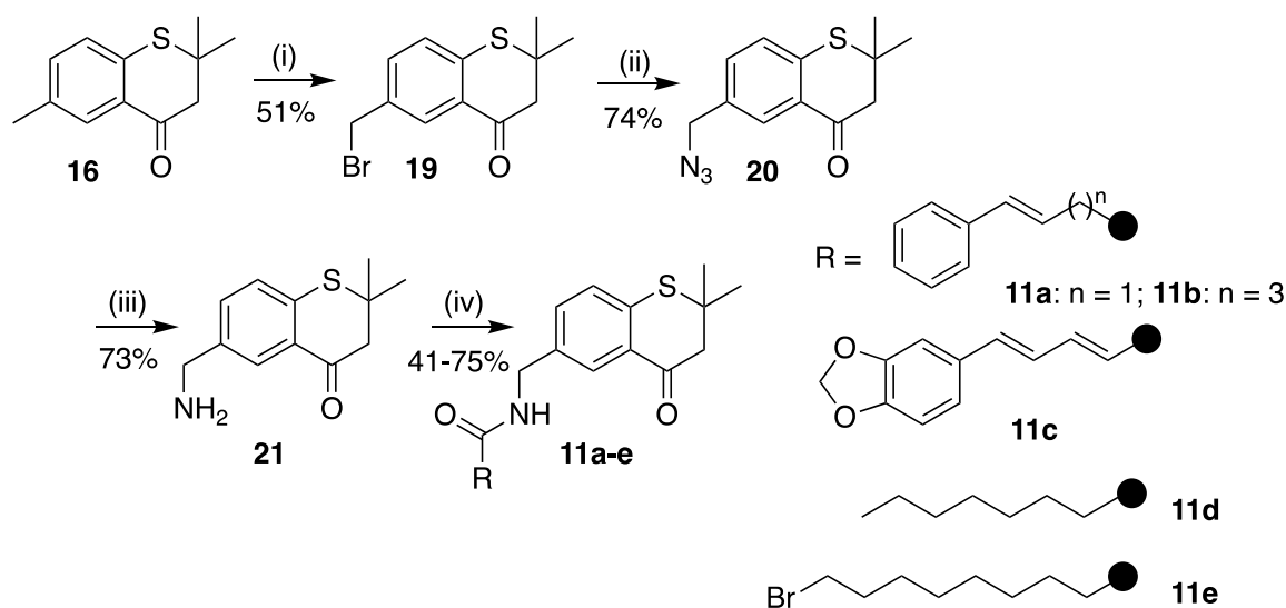
Scheme 2. Synthesis of compounds 11a–e . Reagents and conditions: (i) NBS, dibenzoyl peroxide, cyclohexane, 95\text{--}100^\circ\text{C} , 8 h; (ii) \text{NaN}_3 , DMF, 50^\circ\text{C} , 3 h; (iii) \text{PPH}_3 , \text{THF}/\text{H}_2\text{O} (10:1), RT, 12 h; (iv) \text{RCOOH} , EDC, \text{Et}_3\text{N} , RT, 24 h.
