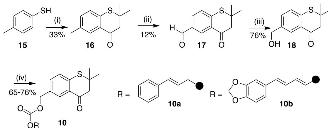
Scheme 1. Synthesis of compounds 10a,b . Reagents and conditions: (i) (\text{CH}_3)_2\text{C}=\text{CHCOOH} , \text{MeSO}_3\text{H} , 80^\circ\text{C} , 8 h; (ii) \text{K}_2\text{S}_2\text{O}_8 , \text{CuSO}_4 , \text{H}_2\text{O}/\text{CH}_3\text{CN} (1:1), 75\text{--}80^\circ\text{C} , 1 h; (iii) D. carota , RT, 72 h; (iv) Appropriate acid, EDC, \text{Et}_3\text{N} , DCM, 0^\circ\text{C} –RT, 24–72 h.
