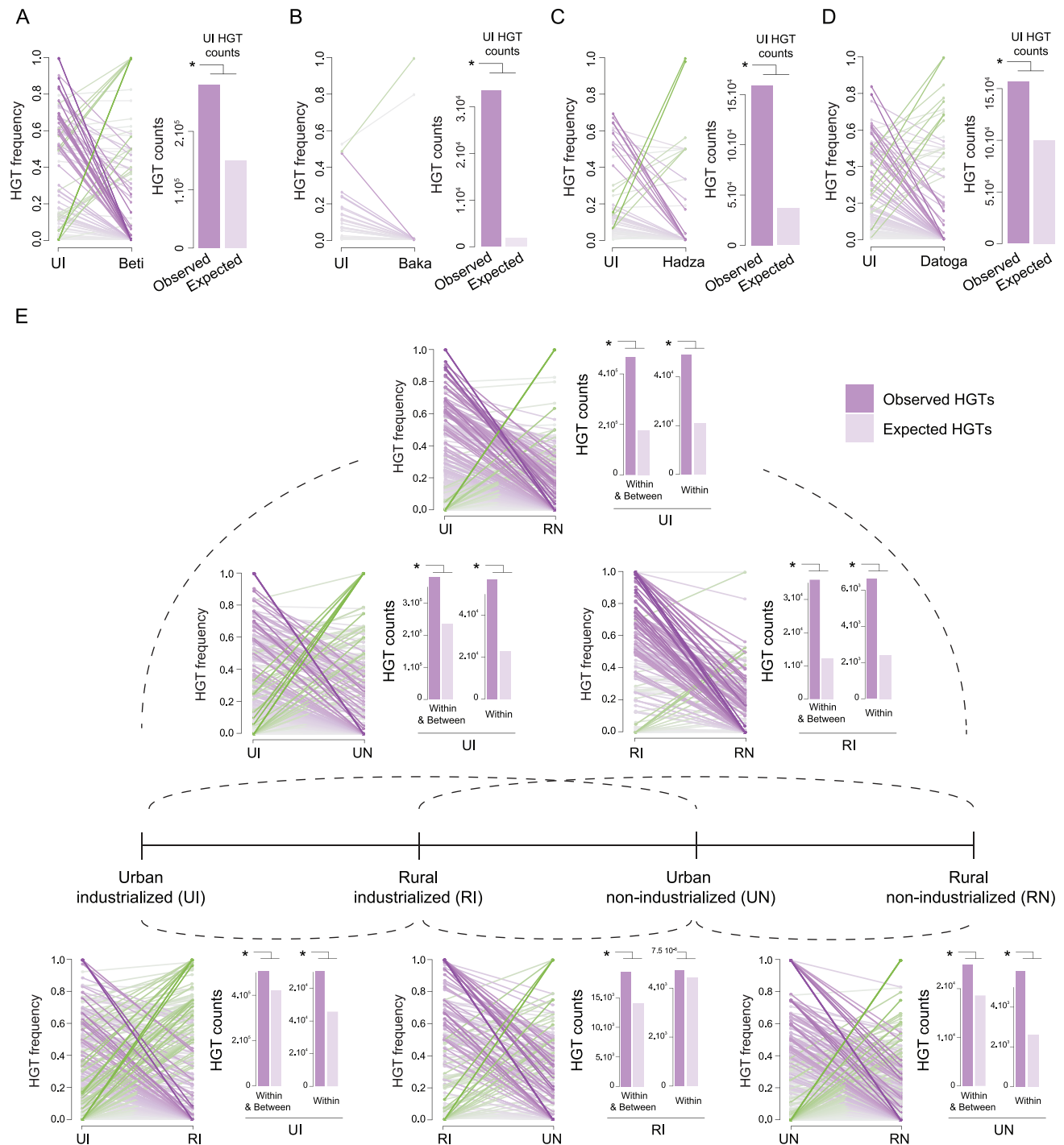
Figure S5. Elevated HGT frequency in the gut microbiome of individuals living in industrialized and urban populations, related to Figures 4B and 4C
