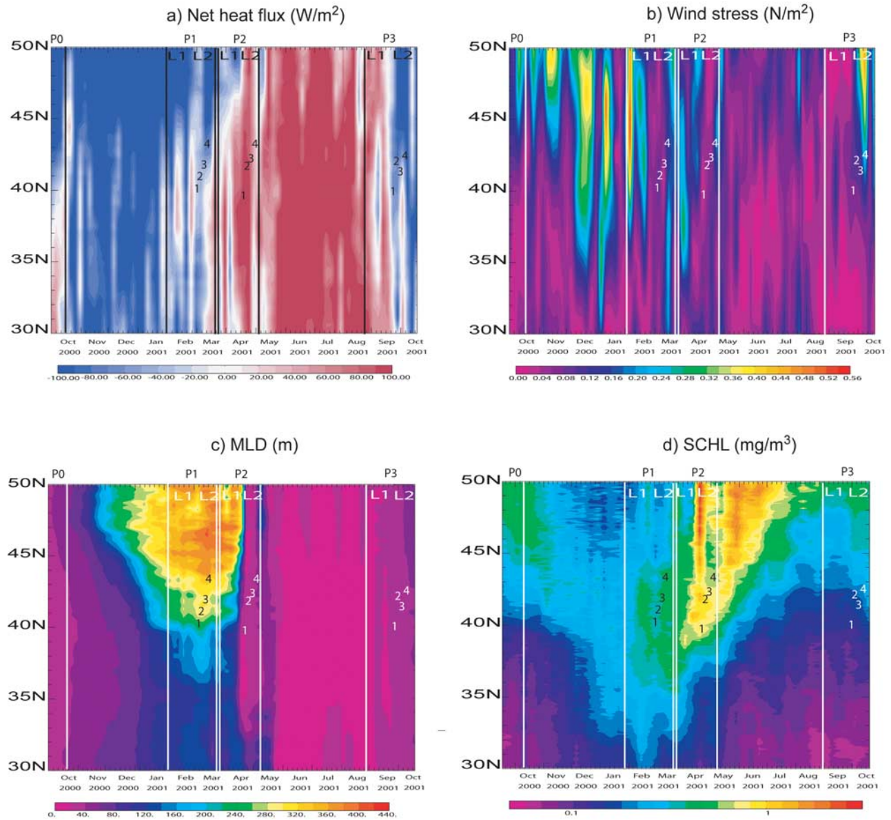
Figure 2. Temporal and meridional variations of zonal averages ( 16^{\circ} – 22^{\circ}\text{W} ) from September 2000 to October 2001 of (a) net heat flux (Clipper), (b) wind stress (ECMWF), (c) MLD (Clipper), and (d) SCHL (SeaWiFS). The vertical lines mark the period of each POMME survey (P0 to P3). The numbers mark the location and time of the time series stations. Legs 1 (L1) and 2 (L2) of each survey are also indicated.
