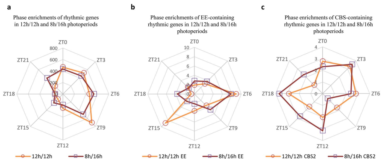
Figure 6. Time-dependent enrichment in core clock elements for both photoperiods: (a) radar chart that represents the number of rhythmic genes with a maximum value of the expression level through photoperiod 12 h/12 h (orange line) and 8 h/16 h (purple line). (b, c) Radar charts that represent the number of rhythmic genes containing cis -regulatory modules (EE and CBS) with the maximum value of the expression level through photoperiod 12 h/12 h (orange line) and 8 h/16 h (purple line).
