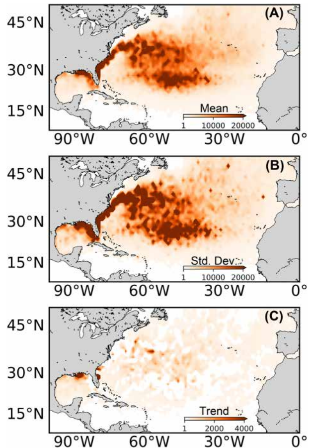
Figure 4. Maps of predicted oceanic-stage loggerhead turtle density derived from dispersal simulations weighted by estimates of hatching production and survival from 1996 through 2017 in 1^\circ latitude \times 1^\circ longitude bins. (A) Depicts the mean annual number of turtles in each bin. (B) Shows the absolute value of the annual standard deviation of mean density. (C) Indicates the increase in the number of turtles each year (positive trend) by location.
