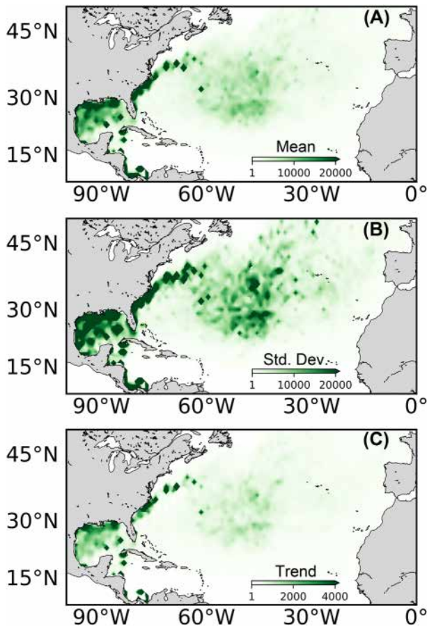
Figure 3. Maps of predicted oceanic-stage green turtle density derived from dispersal simulations weighted by estimates of hatching production and survival from 1996 through 2017 in 1^\circ latitude \times 1^\circ longitude bins. (A) Depicts the mean annual number of turtles in each bin. (B) Shows the absolute value of the annual standard deviation of mean density. (C) Indicates the increase in the number of turtles each year (positive trend) by location.
