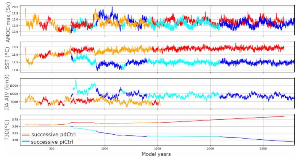
Figure 3. Time evolution of the AMOC maximum taken between 10 and 60°N (top panel), global mean SST (second panel), summer Arctic sea ice volume (third panel) and global mean averaged oceanic temperature (bottom panel) of the successive configurations starting from the last one (first on the left) that was restarted from the Levitus climatology (Locarnini et al., 2013) at rest. The orange and red curves are for the successive pdControl configurations. The first present-day simulation considered here is a tuned version of CM6.0.11-pd. The light and dark blue curves are for the successive piControl simulations. The first preindustrial control simulation was started from CM6.0.12-pd. Note that although, from this version onward, all changes applied to the pdControl configurations were systematically also applied to corresponding piControl simulations, there may have been some intermediate pdControl versions before changes were applied to piControl and all configurations were not integrated for rigorously the same length. This explains that there is not exact matching between the succession of pdControl and piControl versions.
