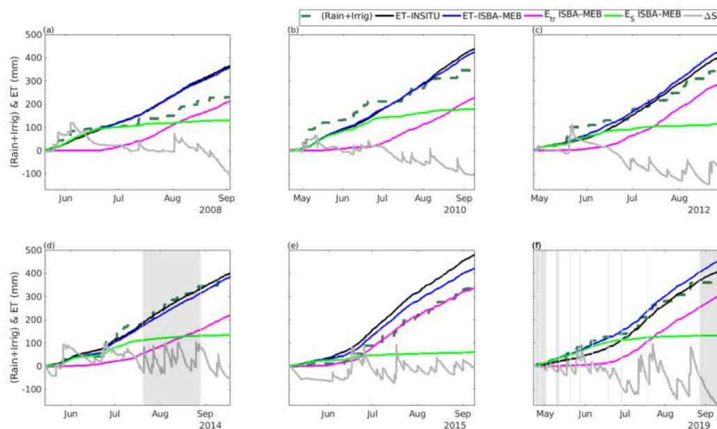
Figure 11. Comparing the cumulated rainfall (+irrigation) with evapotranspiration (ET) from field measurements and ISBA-MEB estimates with plant transpiration ( E_{tr} ), soil evaporation ( E_s ), and soil water storage ( \Delta S ) for the maize seasons at FR-Lam site. The grey area in the chart represents periods without soil water measurements and periods substituted with ISBA-MEB measurements.
