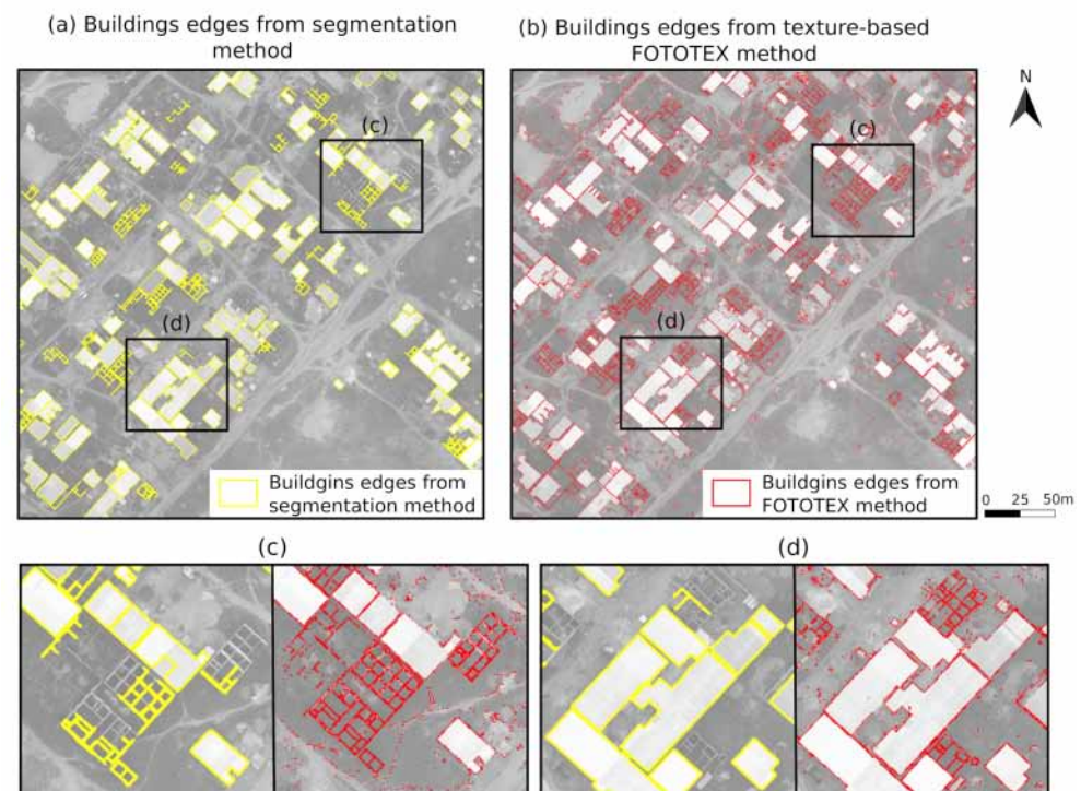
Figure 13. Extraction of buildings edges with (a) a segmentation method carried out with the Large Scale Generic Region Merging algorithm (Orfeo Toolbox) and (b) the FOTOTEX method implemented on the blue band of UAV image. (c,d) zooms on two different areas to compare detection by FOTOTEX and segmentation.
