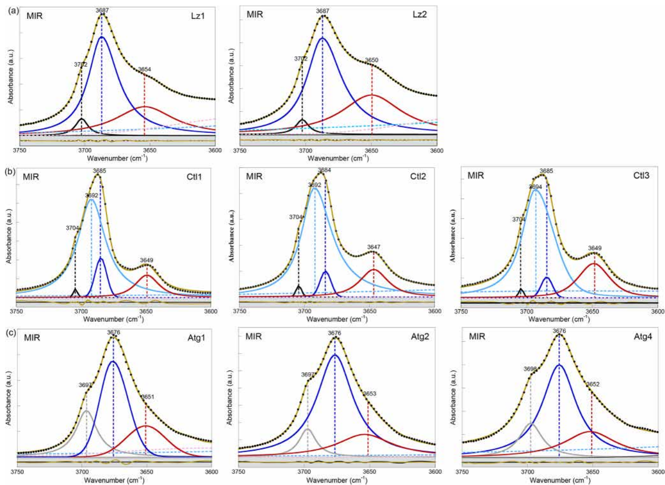
Figure A2. MIR spectra in the 3750–3600 cm -1 range (first overtone region of OH stretching bands) of (a) lizardite (Lz1, Lz2), (b) chrysotile (Ctl1, Ctl2, Ctl3), and (c) antigorite (Atg1, Atg2, Atg4). The spectra have been decomposed into individual components using asymmetric Lorentzian–Gaussian functions. Black dots: experimental data. Solid brown line: best fit (residues in bottom grey box). Plain black and grey curves: inner OH stretching modes. Plain blue and red (or purple) curves: interlayer OH stretching modes. Dashed pink and light blue curves: H 2 O vibration modes.
