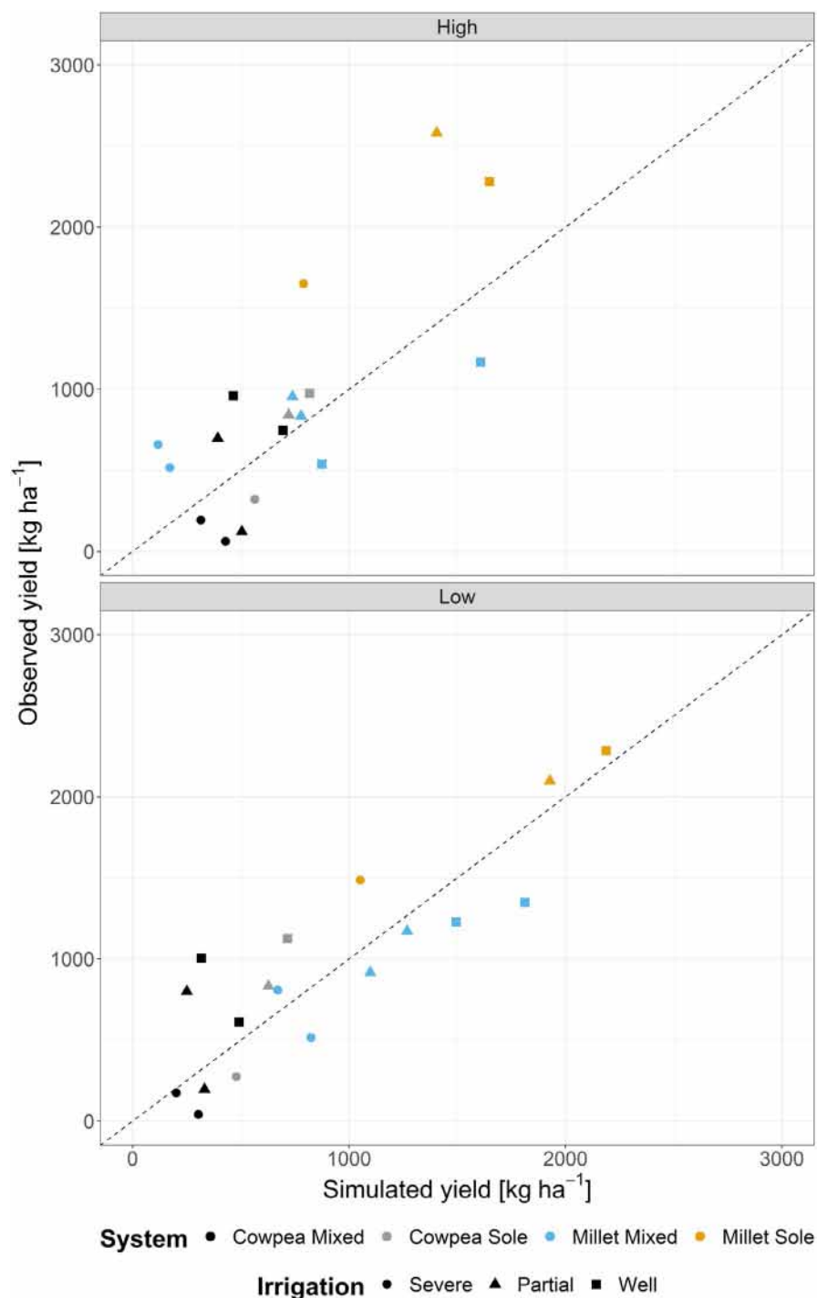
FIGURE 4 Simulated (x-axis) versus observed (y-axis) grain yield for cowpea and pearl millet sole crops and intercropped stands with high, 33, and low, 17 plants per \text{m}^{-2} planting densities in Patancheru—plots top and bottom respectively. Colours represent the cropping system; and shape the weekly irrigation treatments: severe, until pearl millet flowering (circles), partial, until cowpea flowering (triangles), and well-watered, until two weeks after cowpea flowering (squares)
