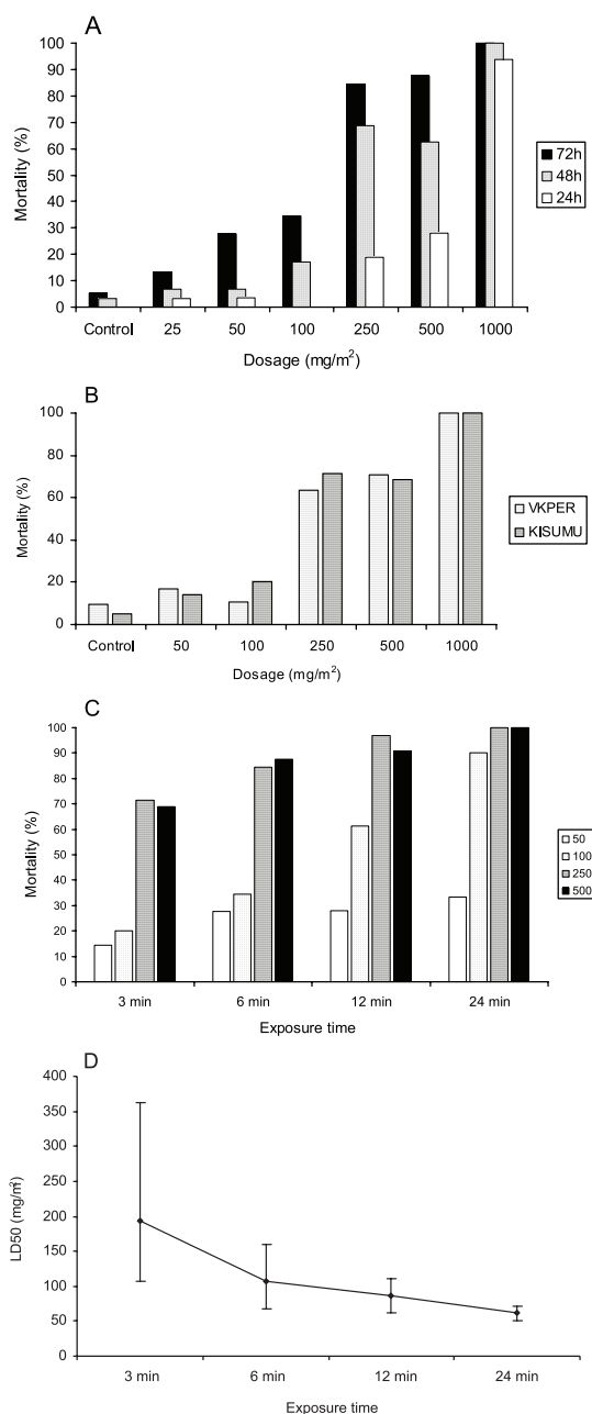
Fig. 1. Efficacy of indoxacarb-treated netting across a range of dosages against An. gambiae in WHO cone assays. (A) Delayed mortality of the Kisumu strain after 3-min exposure to treated netting. (B) Mortality of Kisumu and VKPER strains 72 h after the initial 3-min exposure to treated netting. (C) Mortality of the susceptible Kisumu strain across a range of dosages and exposure times. (D) LD 50 s \pm CIs of the insecticide-susceptible Kisumu strain after exposure to treated netting for various exposure times.
