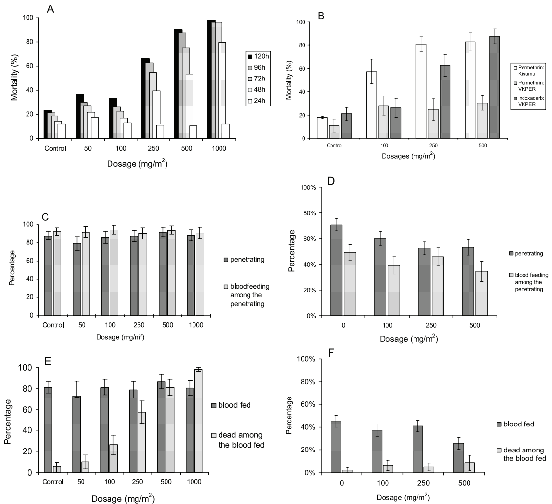
Fig. 2. Efficacy of indoxacarb and permethrin treated netting against An. gambiae in tunnel tests. (A) Delayed mortality to indoxacarb over 24 h to 120 h (VKPER strain). (B) Dosage-mortality response of VKPER and Kisumu strains to permethrin and indoxacarb. Mortality was scored after 24 h in permethrin tests and after 96 h in indoxacarb tests. (C) Proportion penetrating the holed indoxacarb-treated netting and proportion of blood feeding among those that penetrated (VKPER). (D) Proportion penetrating the holed permethrin-treated netting and proportion blood feeding among those that penetrated (VKPER). (E) Indoxacarb tests on VKPER: proportion blood feeding and proportion dead after 48 h among those that blood fed. (F) Permethrin tests on VKPER: proportion blood feeding and proportion dead after 48 h among those that blood fed.
