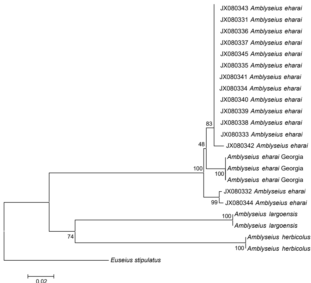
Figure 1 Neighbour joining phylogenetic tree including Amblyseius eharai from Georgia, specimens of Amblyseius eharai , Amblyseius largoensis and A. herbcicolus from Genbank and Euseius stipulatus (as an outgroup) obtained with COI mtDNA fragment.
