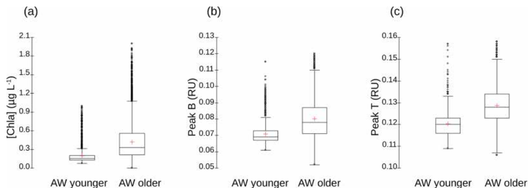
Figure A5. Box-and-whisker plots for the comparison of ( a ) [chl a ] (in micrograms per liter), ( b ) fluorescence intensities of tyrosine-like fluorophore (peak B in RU) and ( c ) fluorescence intensities of tryptophan-like fluorophore (peak T in RU) between younger and older AW. The bottom and top of the box are the 25th and 75th percentiles, respectively, whereas the central line is the 50th percentile (the median), and the cross is the mean. The ends of the error bars correspond to the 10th percentile (bottom) and to 90th percentile (top). All the SeaExplorer glider transects are considered here (all data acquired from 6 to 15 May 2018). Younger AW corresponds to samples showing salinity between 37.20 and 37.84 and temperature between 14.5 and 17.4 °C ( n = 1657 ). Older AW corresponds to samples with salinity between 37.82 and 38.14 and temperature between 14.0 and 18.3 °C ( n = 11\,760 ). Mean values of chl a , peak B and peak T of older AW are significantly higher than those of younger AW ( t test, p < 0.0001 ).
