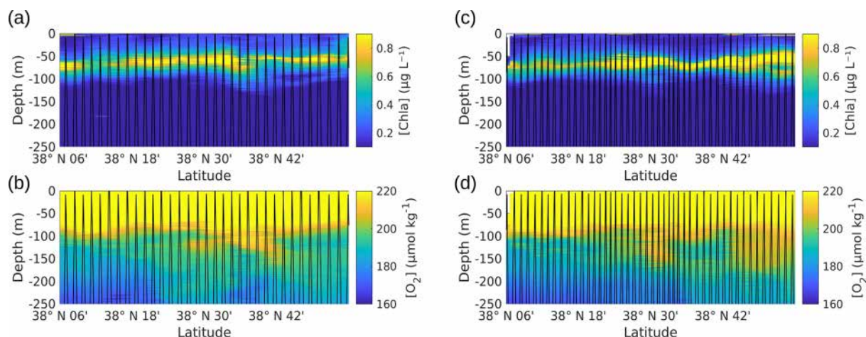
Figure A4. Vertical profiles of [chl a ] ( a , c ) and dissolved oxygen concentration ( b , d ), measured by the SeaExplorer glider, along the outward route ( a , b ) from 6 May 2018 at 00:00 to 9 May 2018 at 21:00 UTC and along the return route ( c , d ) from 10 May 2018 at 00:00 to 13 May 2018 at 21:00 UTC. The SeaExplorer glider trajectory is depicted by the black lines. The data were selected between the surface and 250 m for a better visualization of the surface layer.
