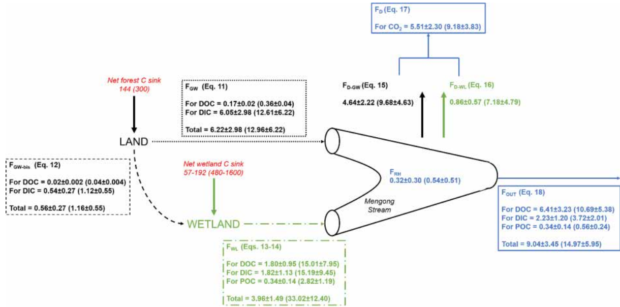
Figure 7. Mass balance of C in the first-order Mengong catchment. All fluxes are in MgC yr -1 , and in MgC km -2 yr -1 when between brackets (weighed by the surface area of 0.48 km 2 drained by non-flooded forest groundwater for the net forest C sink, F_{GW} , F_{GW-bis} and F_{D-GW} ; by the wetland surface area of 0.12 km 2 for the net wetland C sink, F_{WT} and F_{D-WL} ; and by the Mengong catchment area of 0.6 km 2 for F_{OUT} , F_D and F_{RH} ), and they are associated with their corresponding equations as described in detail in the Sect. 2.5. Briefly, F_{GW} is the quantity of dissolved carbon leached from non-flooded forest groundwater to the Mengong stream (Eq. 11), F_{GW-bis} is the quantity of dissolved carbon leached from non-flooded forest groundwater to the Mengong wetland (Eq. 12), F_{WL} is the quantity of carbon leached from the Mengong wetland to the Mengong stream (Eqs. 13–14), F_D is the quantity of C degassed from the Mengong stream to the atmosphere, F_{RH} is the heterotrophic respiration in the Mengong stream and F_{OUT} is the quantity of carbon hydrologically exported at the outlet of the Mengong stream. In addition, net forest C sink of the Mengong catchment estimated by Brunet et al. (2009) and a range of typical net wetland C sink measured in wetlands in Africa by Saunders et al. (2007) and Jones and Humphries (2002) are both indicated.
