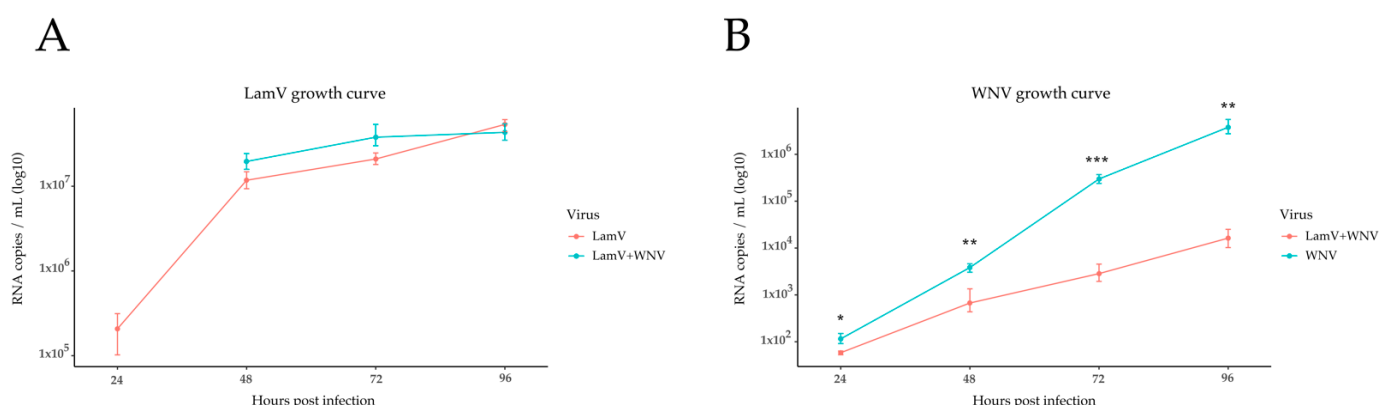
Figure 1. Growth curves of LamV and WNV in U4.4 cells, shown as RNA copies/mL over time. (A) LamV growth curve. (B) WNV growth curve. Dots show the mean RNA copy number per mL with a standard deviation among the biological replicates. * p < 0.05 , ** p < 0.01 , *** p < 0.001 .
