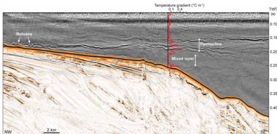
Figure 11. Multi-channel high-resolution seismic reflection profile MOZ04-HR-117 of the water column (greyscale) and the sub-seafloor (colour scale), and temperature gradient profile collected at the same time. Note the good correlation between high amplitude reflections in the water column and peaks in temperature gradient. [Colour figure can be viewed at wileyonlinelibrary.com ]
