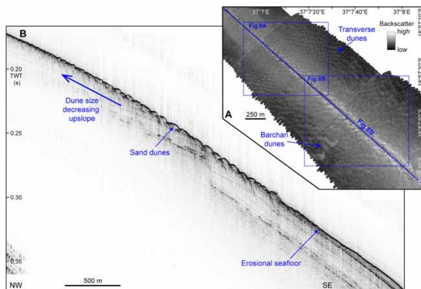
Figure 8. (A) Seafloor backscatter of the dune field. (B) Sub-bottom profiler image MOZ04-SBP-102a along the dune field, showing an erosional seafloor at the foot of the dune field and upslope migrating dunes. [Colour figure can be viewed at wileyonlinelibrary.com ]
