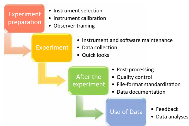
Fig. 4 Data quality control in DACCIIWA experiment preparation, data collection, processing, archiving and sharing.
