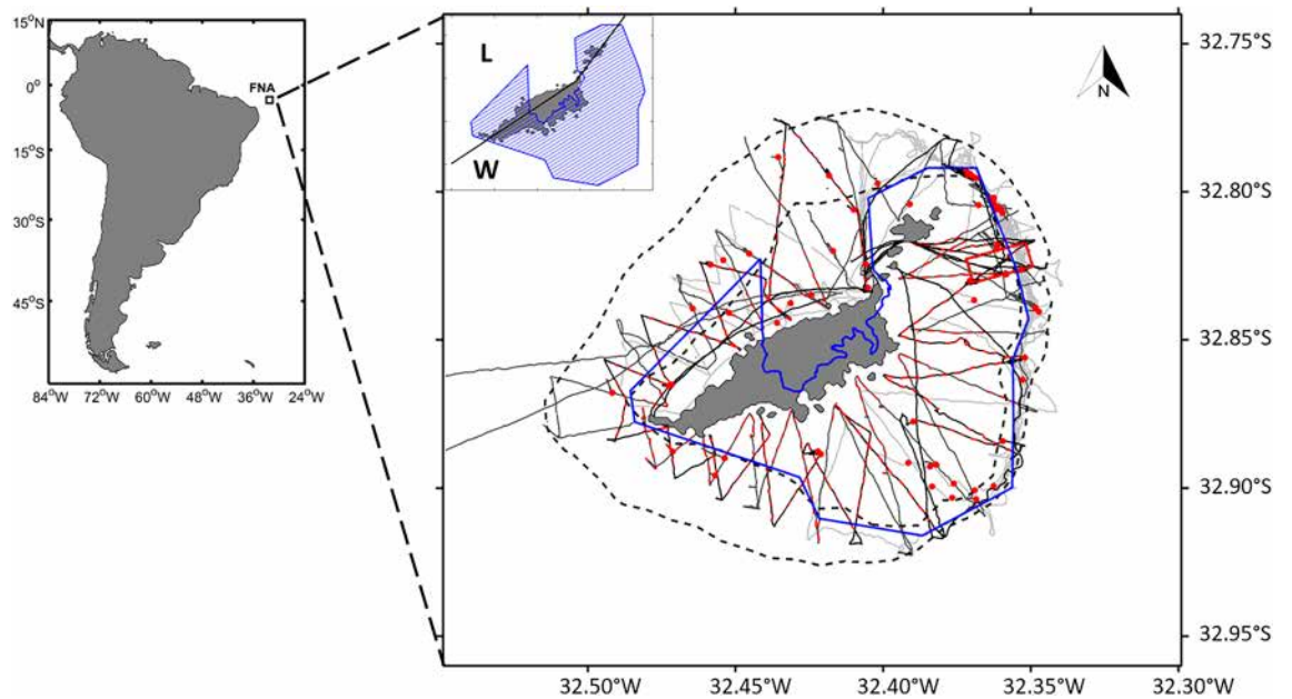
Figure 1. Fernando de Noronha archipelago (FNA) (03°51'S, 32°25'W). The blue line delimits the no take MPA PARNAMAR. Acoustic transects are depicted by light grey (FAROFA 1), dark grey (FAROFA 2) and black lines (FAROFA 3); video transects by red dashed lines and video stations by red dots. The black dashed lines depict the 50 and 300 m isobaths. The insert on the main map show the PARNAMAR hatched in blue and the black solid line separates the leeward side (L) and the windward side (W). Map was created by the authors using Matlab R2018b ( https://fr.mathworks.com/ ) and m_map mapping package 84 .
