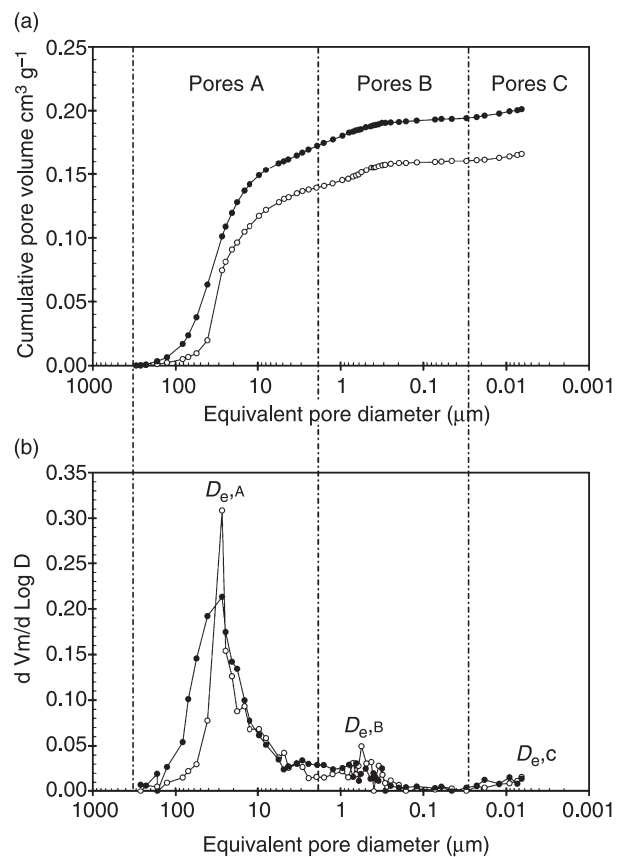
Figure 4 Cumulated mercury intrusion curve (a) and its derivative curve (b) recorded for the E horizon (—○—) and E_{slot} material (—●—).
