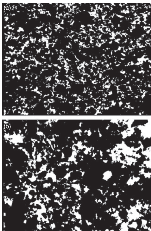
Figure 5 Binary image of the porosity in the E horizon (a) and in the E_{\text{slot}} material (b) (pores analysed by image analysis are in white, the original size was 7.7 \times 5.7 \text{ mm}^2 ).
