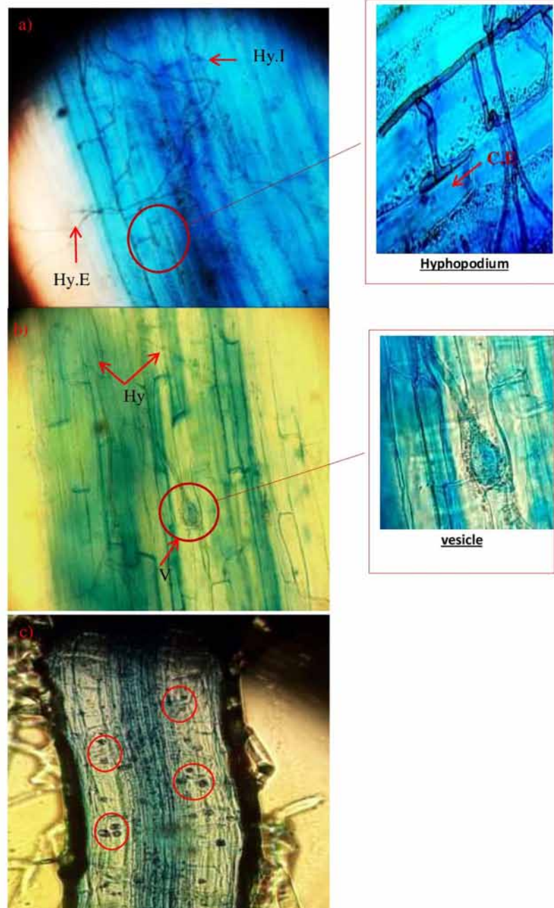
FIGURE 6 | Evolution of AMF structure, hyphae, as well as the presence of a hyphopodium in wheat plants (Hy.E: extra root hyphae; Hy.I: intra-root hypha; CE: epidermal cell; V: vesicle) ( \times 400 ).
