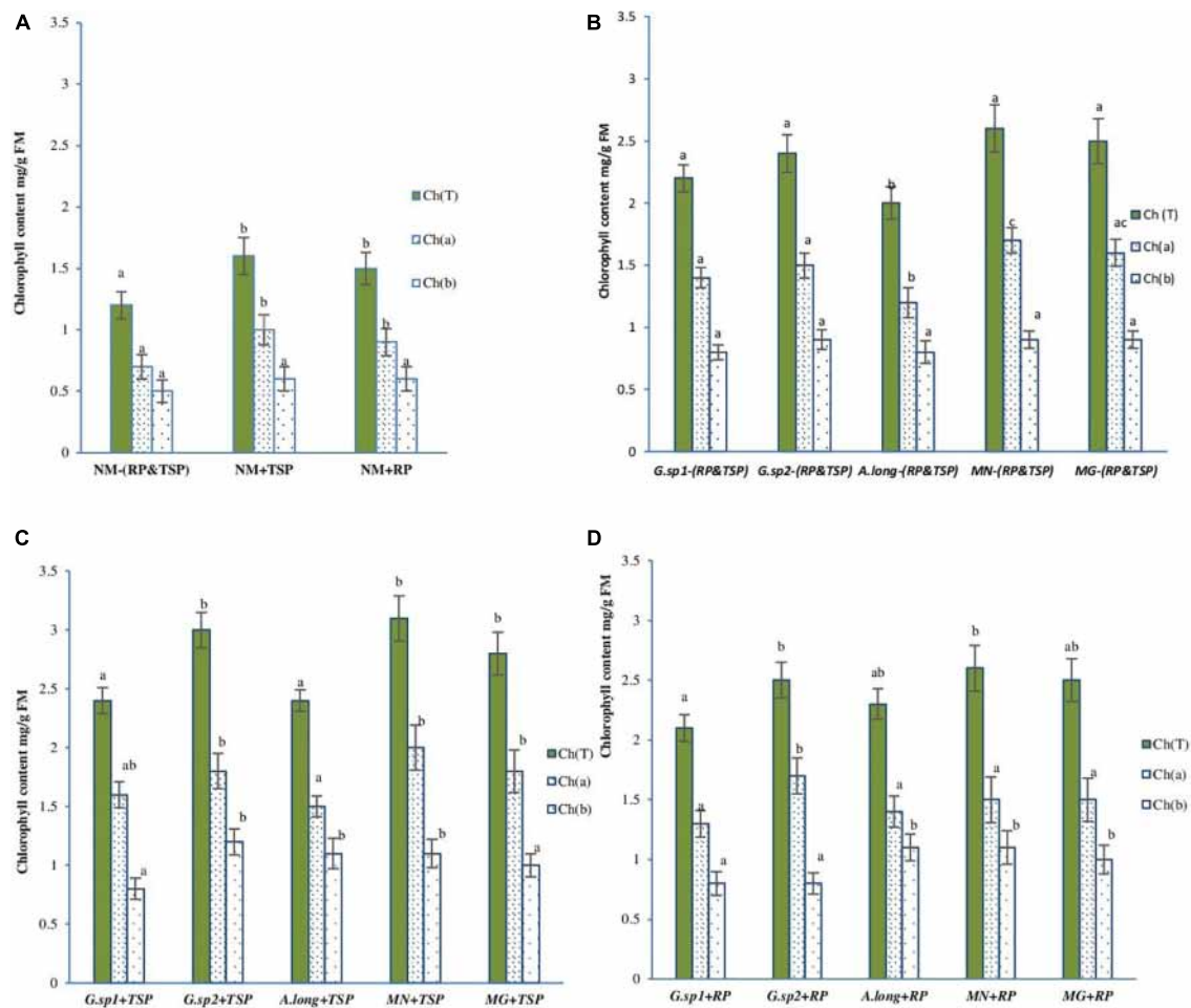
FIGURE 8 | Chlorophyll (a,b and total) content variation in wheat plant with the presence of AMF, and TSP & RP in the medium: (A) non-mycorrhizal plants (NM), (B) mycorrhizal plants with the four inoculum and the absence of any phosphate sources M-TSP, -RP, (C) mycorrhizal plants with the four morphotype with the presence of TSP free phosphate sources (M + TSP), (D) mycorrhizal plants with the four morphotype with the presence of RP phosphate sources M + RP. The values followed by different letters are significantly different ( P = 0.05 ).
