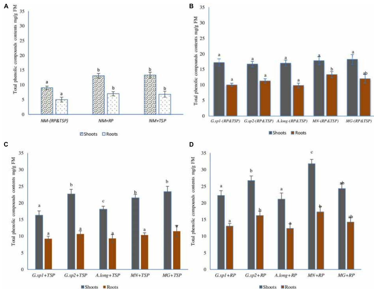
FIGURE 9 | Total phenolic compound content in wheat plant according to the presence of AMF, and the presence of TSP & RP in the medium: (A) non-mycorrhizal plants, (B) mycorrhizal plants with the four inoculum and the absence of any phosphate sources, (C) mycorrhizal plants with the four morphotype with the presence of TSP like free phosphate sources, (D) mycorrhizal plants with the four morphotype with the presence of RP like phosphate sources. The values followed by different letters are significantly different ( P = 0.05 ).
