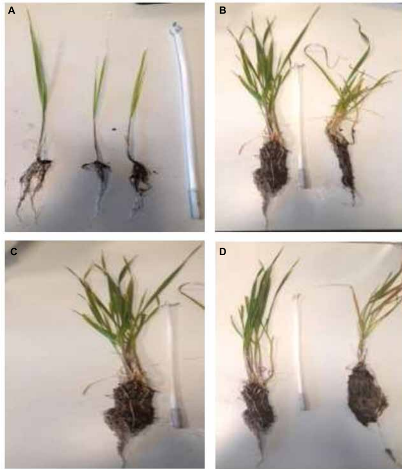
FIGURE 7 | Variation of the growth in the presence and absence of mycorrhizal inoculation, with the presence of RP and TSP: (A) non-mycorrhizal plants; (B) mycorrhizae + TSP and mycorrhizae without (TSP and RP); (C) mycorrhizae + TSP; (D) mycorrhizae + TSP and mycorrhizae + RP (inoculum used: Glomus sp2).
