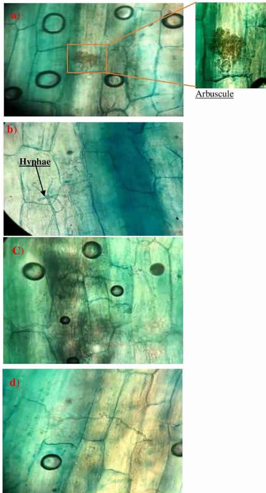
FIGURE 5 | Observations of mycorrhizal structures in Disitaria sanguinalis (a,b) and Alternanthera caracasana (c,d). wild plants in phosphate mines ( \times 400 ).
