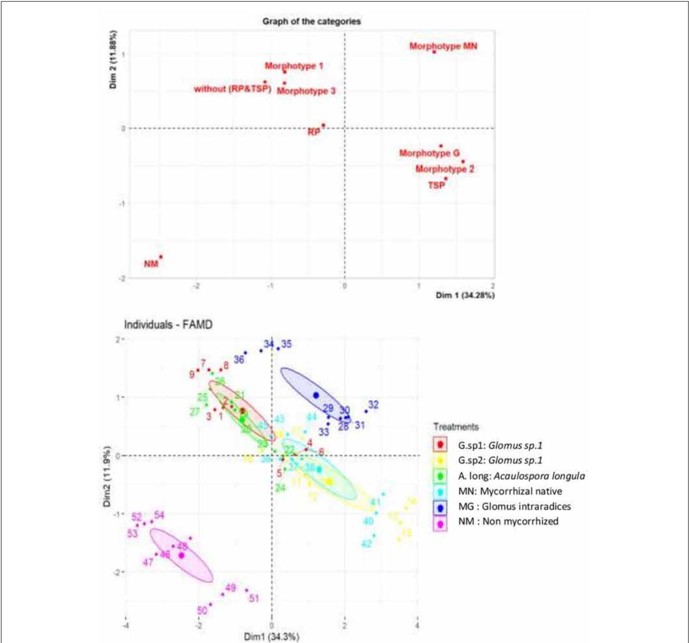
FIGURE 10 | Principal component analysis of wheat plant according to the presence/absence of AMF, TSP & RP in the medium and also the impact of each inoculum and P source on chlorophyll content, stems, and roots growth.
