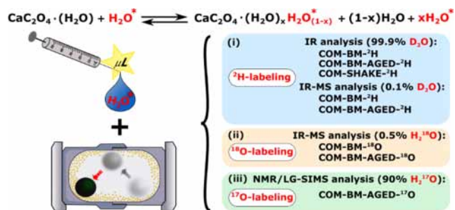
Scheme 1. Schematic Representation of the Mechanochemical Labeling Strategy Together with All Samples Prepared in This Study a
