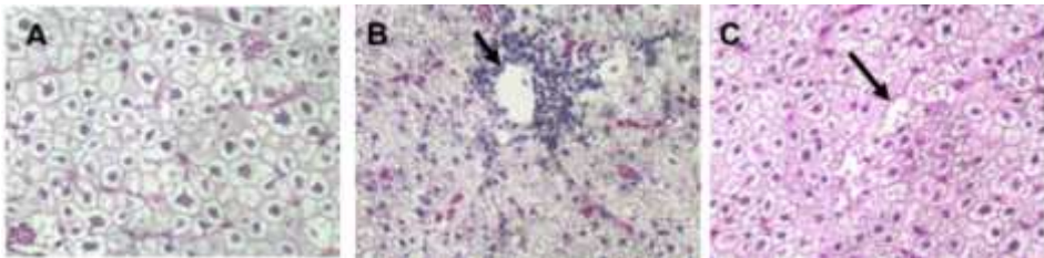
Fig. 2. HE staining of section from samples obtained from carp at 3, 10 dpi and the end of the experiment after cohabitation with TiLV infected tilapia (2017A and 2017B, ip and immersion) with damages (necrosis) of liver tissues.
