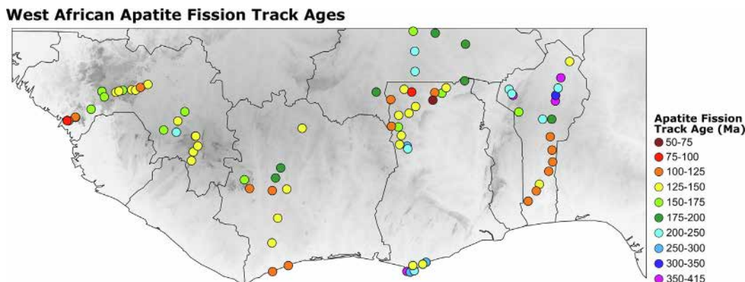
Fig. 8. Maps of West African published AFT data coloured to indicate AFT age. Sample source shown on Fig. 1a.
