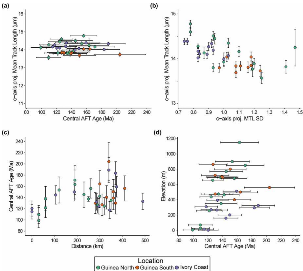
Fig. 3. AFT data plots: (a) c-axis projected mean track length vs. Central AFT age, (b) c-axis projected mean track length vs. c-axis projected mean track length standard deviation, (c) Central AFT age vs. Distance from the coastline, (d) Elevation vs. Central AFT Age. All uncertainties are 1σ.
