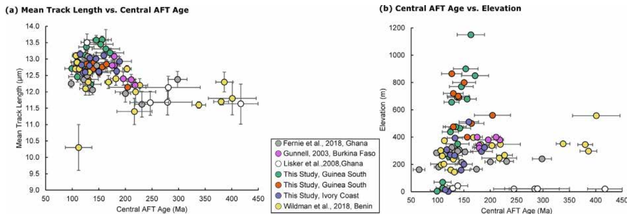
Fig. 7. West African AFT data plots: (a) Mean track length vs. Central AFT age. Measured mean track lengths (i.e., not c-axis projected lengths) are used because c-axis lengths are not presented in all publications) and (b) elevation vs. Central AFT age. All uncertainties are 1 \sigma .
