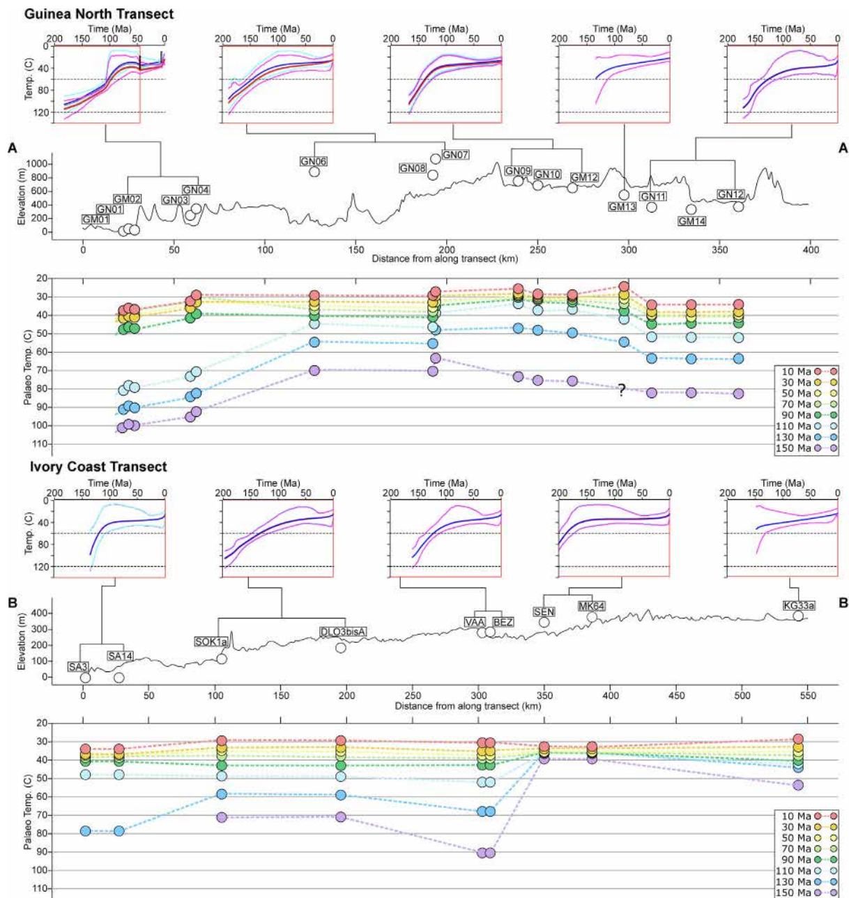
Fig. 5. Topographic profiles for the Guinea North and Ivory Coast transects with sample palaeotemperature at different time periods estimated from the expected thermal history model. Lines of transect are shown on Fig. 2. For clarity, palaeotemperature uncertainties are not shown but can be estimated using the 95% credible intervals on the expected thermal history.
