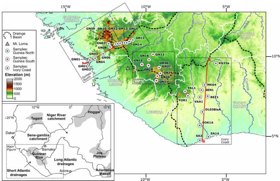
Fig. 2. Topographic map of the Guinea-Ivory Coast region of West Africa showing major rivers and drainage divides, sample locations and lines of transects shown in Fig. 5 and Fig. 6. Inset figure shows West African drainage patterns after Grimaud et al. (2018) and major elevated topographic features.
