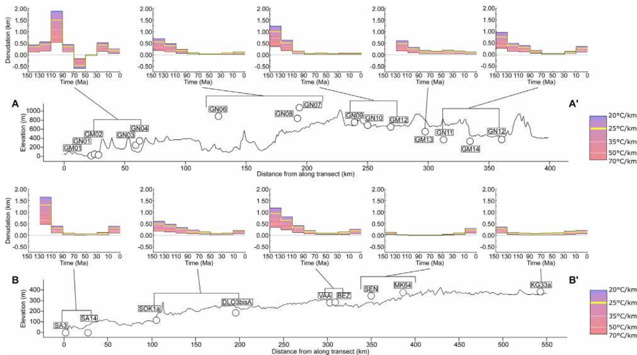
Fig. 6. Topographic profiles for the Guinea North and Ivory Coast transects with estimates of denudation for time intervals: 150 – 130, 130 – 110, 110 – 90, 90 – 70, 70 – 50, 50 – 30, 30 – 10 and 10 – 0 Ma. Yellow line highlights the estimates when a geothermal gradient of 25 °C/km is used. Bars show the range of possible denudation magnitudes for geothermal gradients between 20 and 70 °C/km. Lines of transect are shown on Fig. 2. (For interpretation of the references to colour in this figure legend, the reader is referred to the web version of this article.)
