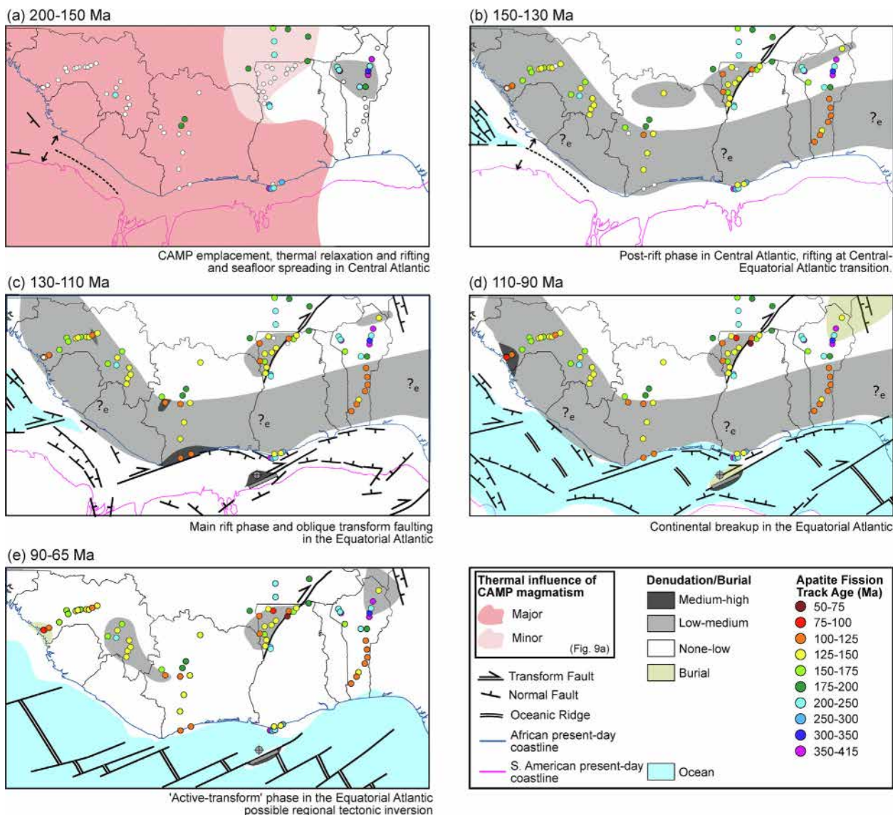
Fig. 9. Maps of West Africa summarising tectonic, thermal, and surface evolution over the Late Jurassic and Cretaceous. Palaeogeography and tectonics structures adopted after Ye et al. (2017). (a) During Late Jurassic the emplacement of the Central Atlantic Magmatic Province caused thermal resetting of samples across Guinea, Ivory Coast and potentially in Ghana. Samples in Benin are not reset and preserve a record of Palaeozoic denudation. (b) Denudation across the length of continental margin in response to rifting in the Equatorial Atlantic. Denudation inland due to erosion of marginal upwarps, inland of drainage divides or erosion of uplifted blocks due to intraplate fault reactivation along the Bole-Nangodi Shear Zone (Fernie et al., 2018). (c) Denudation along coastal margin and across some inland regions continues through late Early Cretaceous at moderate rates, faster denudation observed along the Ivory Coast coastline and the offshore marginal ridge in response to the main phase of rifting and onset of transform faulting in the Equatorial Atlantic. (d) Denudation is generally lower along continental margin during the mid-Cretaceous but enhanced denudation inferred along the Guinean coastline and the southward slope of the offshore Ivory Coast marginal ridge (Bigot-Cromier et al., 2005). Burial inferred inland in Benin along the margins of the Lullemmenden Basin (Wildman et al., 2019) and possibly the northern slopes of the offshore marginal ridge (Clift et al., 1998). (e) Denudation magnitudes are inferred to be low from the Late Cretaceous until present-day. Some interior regions continue to have low-moderate rates of denudation and another phase of intracontinental fault inversion may have occurred.
