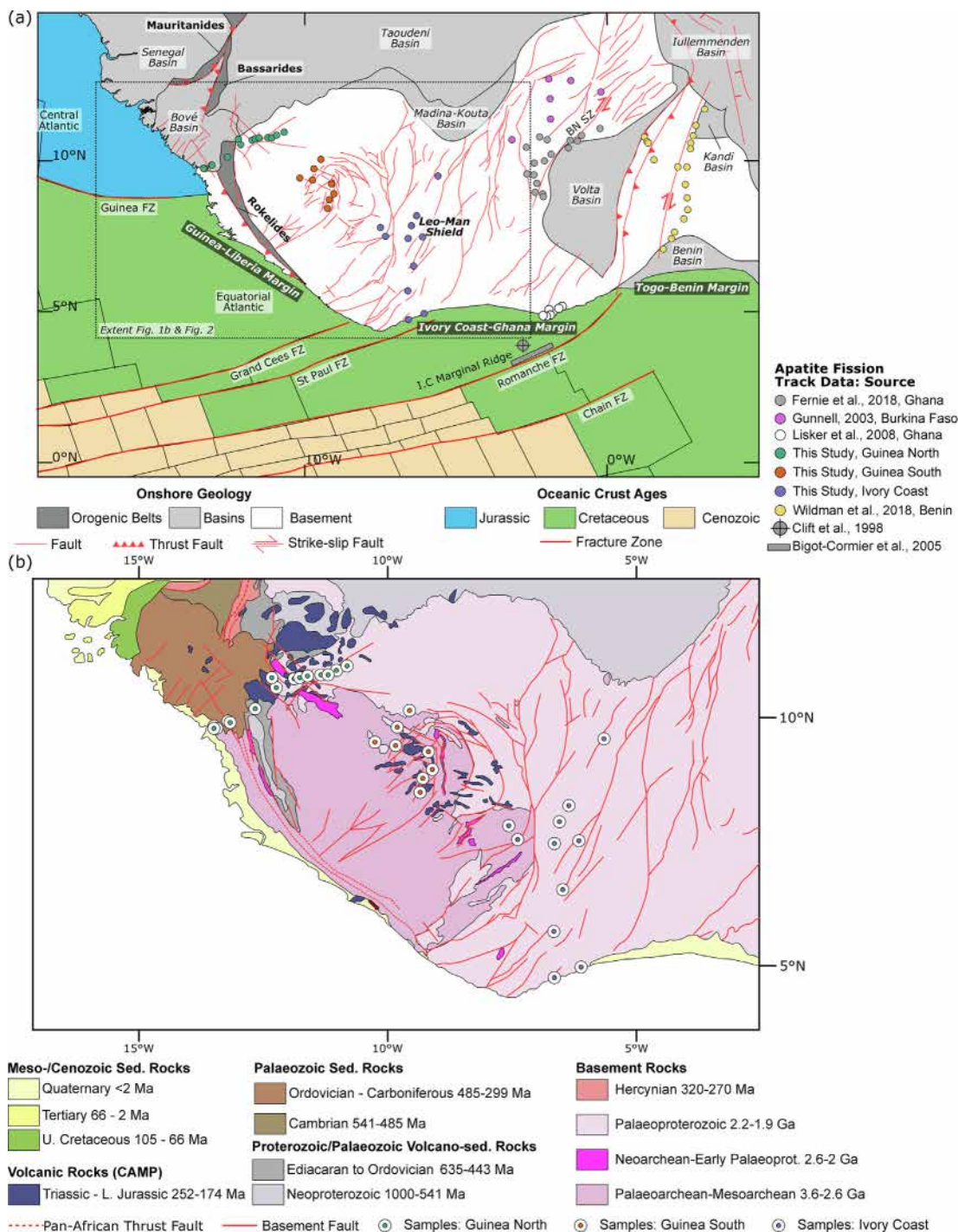
Fig. 1. (a) Tectonic map of West Africa showing major sedimentary basins, deformation belts, faults and Leo-Man cratonic shield onshore and major fracture zones (FZ) and oceanic crust age offshore. BN SZ – Bole Nangodi shear zone. Location of apatite fission-track data, colour coded for their publication are shown. (b) Geology of part of the map area of Fig. 1a showing the location of the samples from Guinea and Ivory Coast presented in this study.
