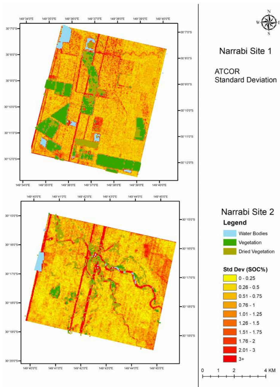
Figure 13. Standard deviation map of estimated SOC obtained along the six WV values used with ATCOR method.
