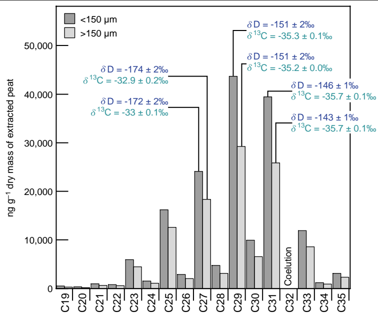
Extended Data Fig. 8 | Concentration, distribution, \delta D and \delta^{13}C of n -alkanes in different size fractions. Coarse fraction >150 μm (including roots) and fine fraction <150 μm were extracted from sample depth 296.5 cm. n -Alkanes in both fractions show similar distribution and have the same \delta D and \delta^{13}C values.
