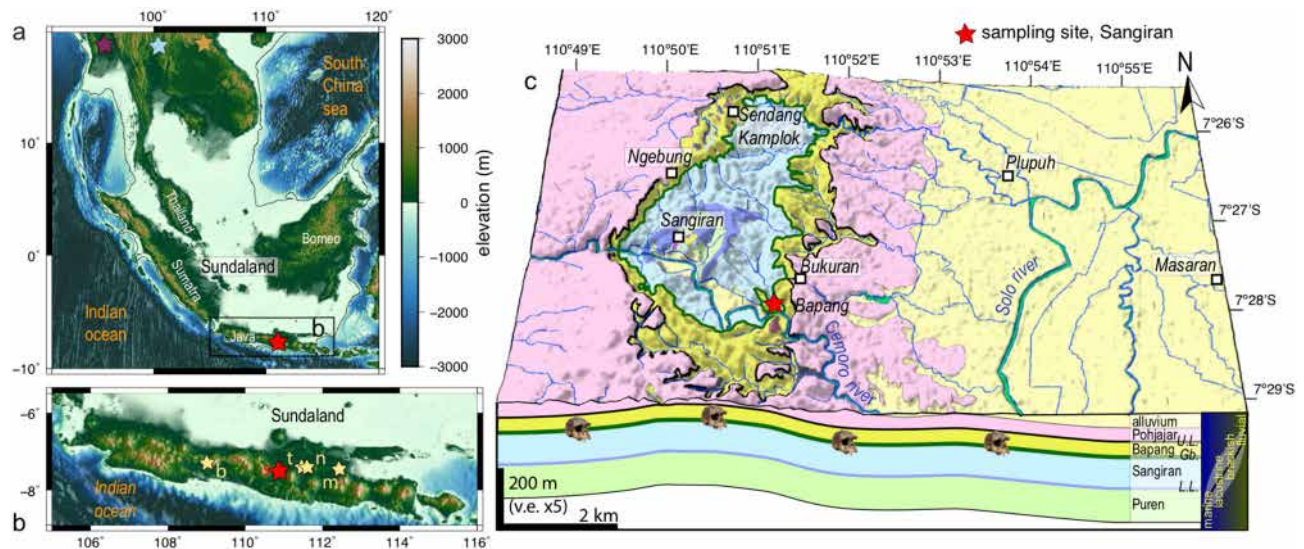
Figure 1. Geology of Sangiran. (a) Regional view. Black line delineates continental Sundaland (120 m isodepth). Stars indicate possible northern entry points (thereafter set to Myanmar, Thailand and Vietnam) for H. erectus . (b) Java island and main biostratigraphic sites (hominin-bearing sites: Sangiran (s), Mojokerto (m), Trinil (t), Ngandong (n); and faunal site Bumiayu (b)). (c) 3D view of the Sangiran dome. Geological map redrawn from 15,22 . Red star locates Bukuran creek outcrop; skull is Sangiran-17 23 . Maps on panels (a,b) were created using GMT 5 ( www.generic-mapping-tools.org ) 24 ; on panel (c), using ArcGIS ( www.arcgis.com ).
