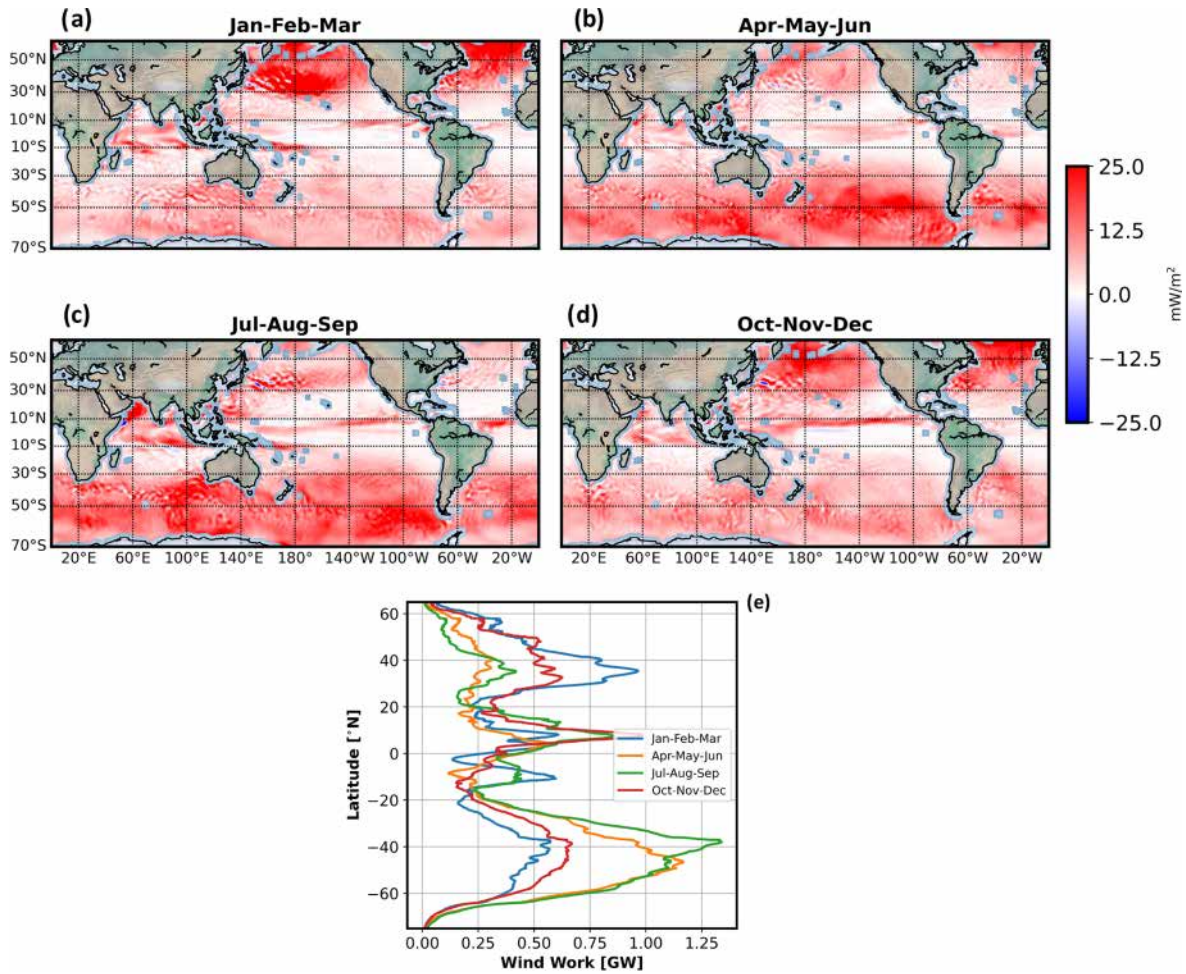
Figure 9. (a–d) Low-frequency wind work with scales larger than L_c averaged over a period of 3 months, \overline{\tau'_{lf} \cdot u'_{o|f}} . (e) Wind work multiplied by the area of the numerical grid cell ( m^2 ) and zonally integrated during four seasons.
