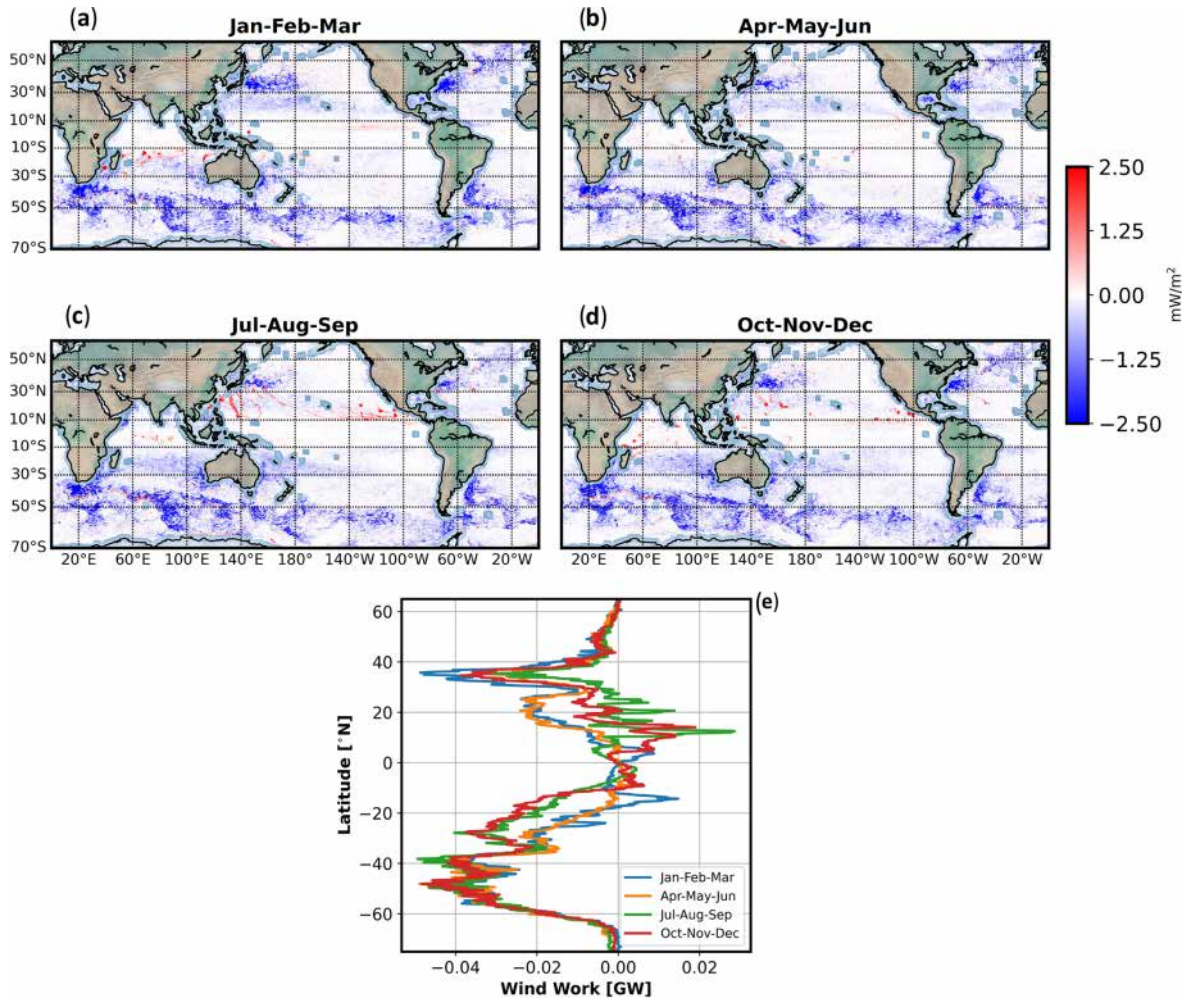
Figure 8. (a–d) Low-frequency wind work with scales smaller than L_c averaged over a period of 3 months, \overline{\tau'_{lf<} \cdot \mathbf{u}'_{0lf<}} . (e) Wind work multiplied by the area of the numerical grid cell ( m^2 ) and zonally integrated during four seasons.
