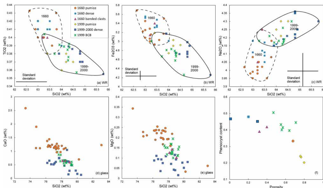
Fig. 2 Composition and phenocryst content of the Guagua Pichincha dacites. a to c Whole rock (WR) composition of the CE 1660 and 1999 products showing the evolution of \text{TiO}_2 , \text{Fe}_2\text{O}_3 and \text{Na}_2\text{O} with \text{SiO}_2 (Samaniego et al. 2010; Wright et al. 2007). d and e Glass composition of pumice clasts of the CE 1660 eruption and breadcrust bombs and dense rocks from the 1999 dome-forming eruption (Sam-
