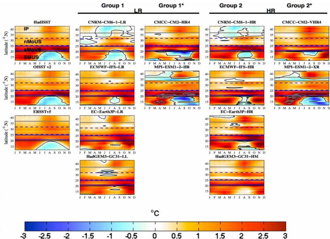
Figure 2. Latitude–time plot of UI^{sst} upwelling index ( ^{\circ}C ) computed as explained in Sect. 2.3. The time axis shows climatological months over the period 1985–2014 for several model configurations and reference data sets (HadISST, OISST v2, and ERSST v5). Models from groups 1, 1*, 2, and 2* respectively (see Sect. 2.1 for the definition of these groups). Positive (negative) values correspond to upwelling (downwelling) conditions. In each panel, the gray line represents the southern boundary of the IP subregion ( 37 – 43^{\circ}N ). The horizontal blue lines (dashed lines) are positioned at 21 and 25^{\circ}N ( 26 and 32^{\circ}N ) and give the limitation of the sMoUS (nMoUS), and the black line represents the northern boundary of the SMUS subregion ( 12 – 20^{\circ}N ). The black (gray) contour shows the contour zero (values > 3^{\circ}C ). This index is calculated over the model’s native grid.
