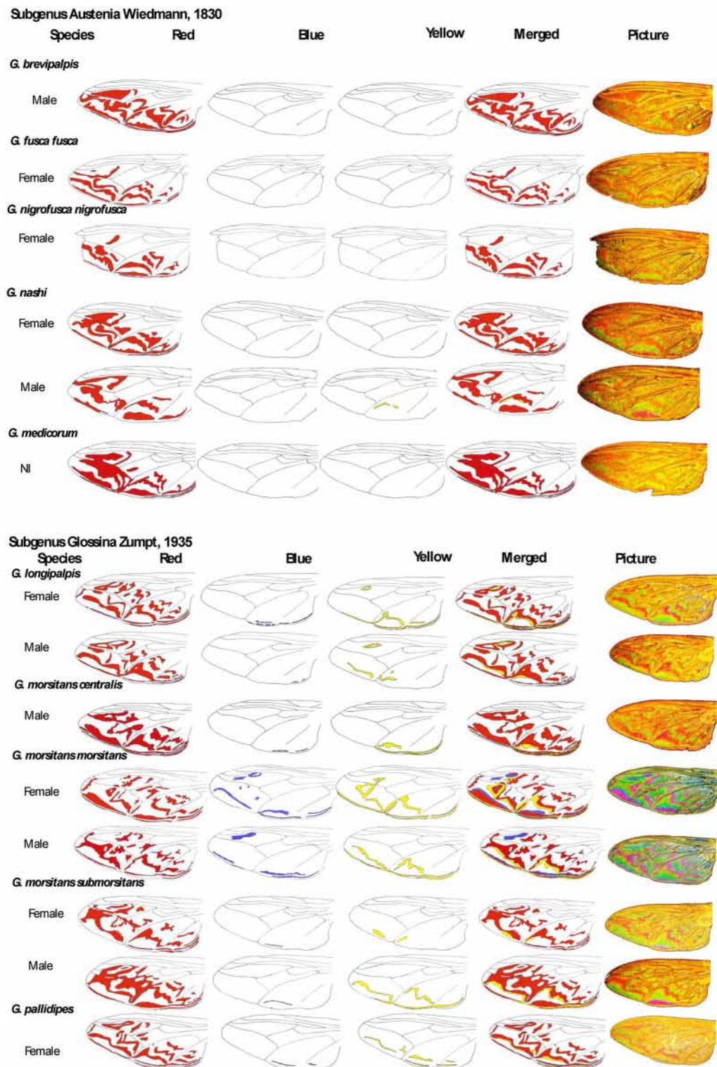
Figure 6. Selected Glossina spp pictorial key, deduced from Wing Interferential Pattern.
