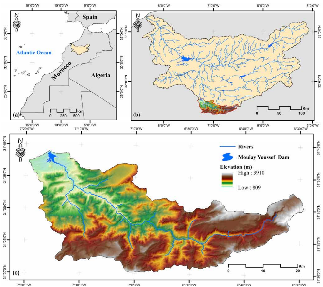
Figure 1. The geographical location of the research region; (a) on Moroccan scale, (b) on Oum Er-Rbia watershed scale, and (c) digital elevation model of the Tassaoute catchment (upstream of the Moulay Youssef Dam).
