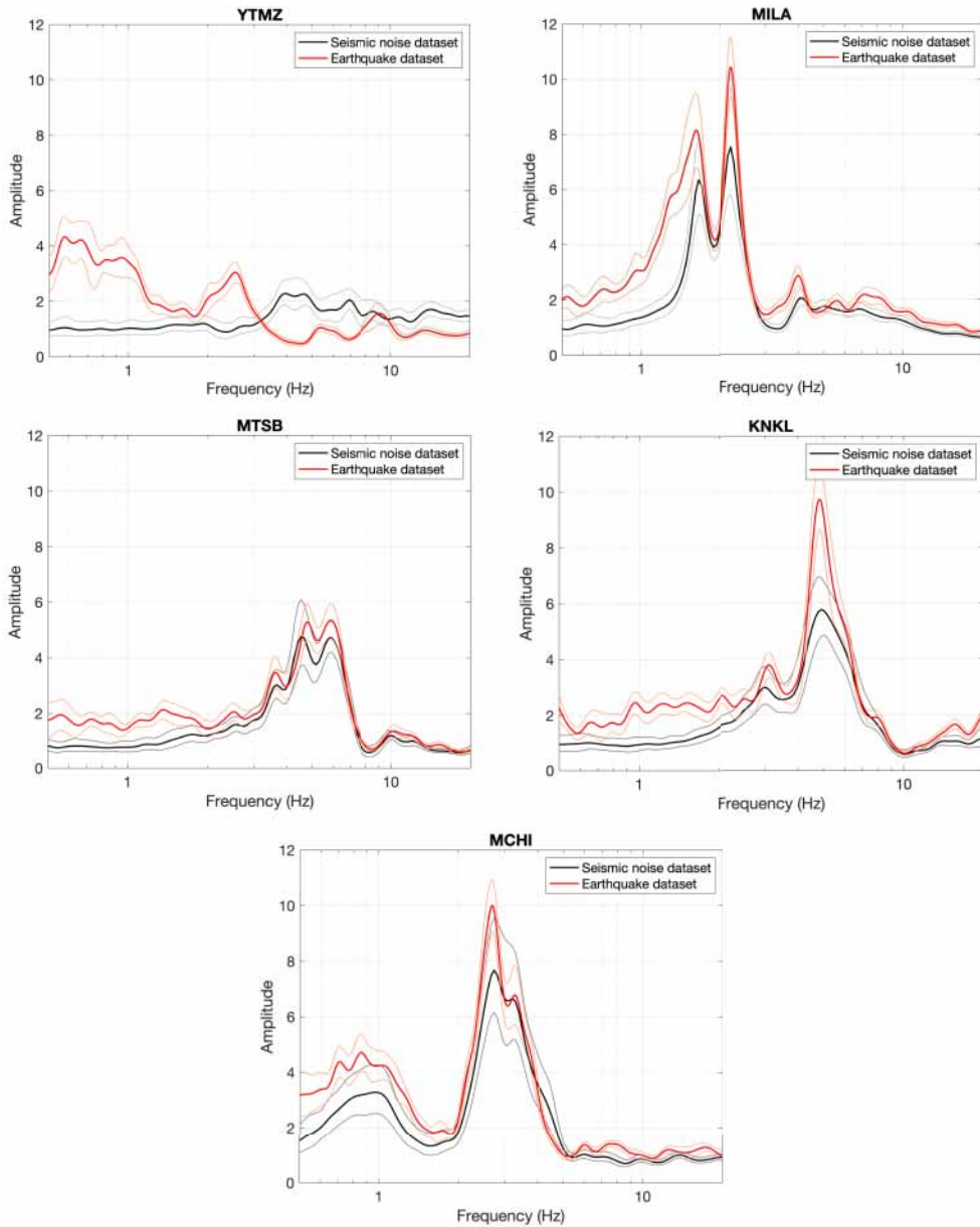
Figure 6. Comparison of H/V spectral ratios performed on earthquake and on seismic noise for stations YTMZ, MILA, MTSB, KNKL and MCHI.
