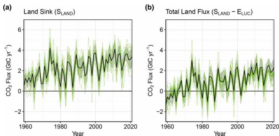
Figure 8. (a) The land CO 2 sink ( S_{LAND} ) estimated by individual DGVM estimates (green), as well as the budget estimate (black with \pm 1\sigma uncertainty), which is the average of all DGVMs. (b) Total atmosphere–land CO 2 fluxes ( S_{LAND} - E_{LUC} ). The budget estimate of the total land flux (black with \pm 1\sigma uncertainty) combines the DGVM estimate of S_{LAND} from panel (a) with the bookkeeping estimate of E_{LUC} from Fig. 7a. Uncertainties are similarly propagated in quadrature from the budget estimates of S_{LAND} from panel (a) and E_{LUC} from Fig. 7a. DGVMs also provide estimates of E_{LUC} (see Fig. 7a), which can be combined with their own estimates of the land sink. Hence, panel (b) also includes an estimate for the total land flux for individual DGVMs (thin green lines) and their multi-model mean (thick green line).
