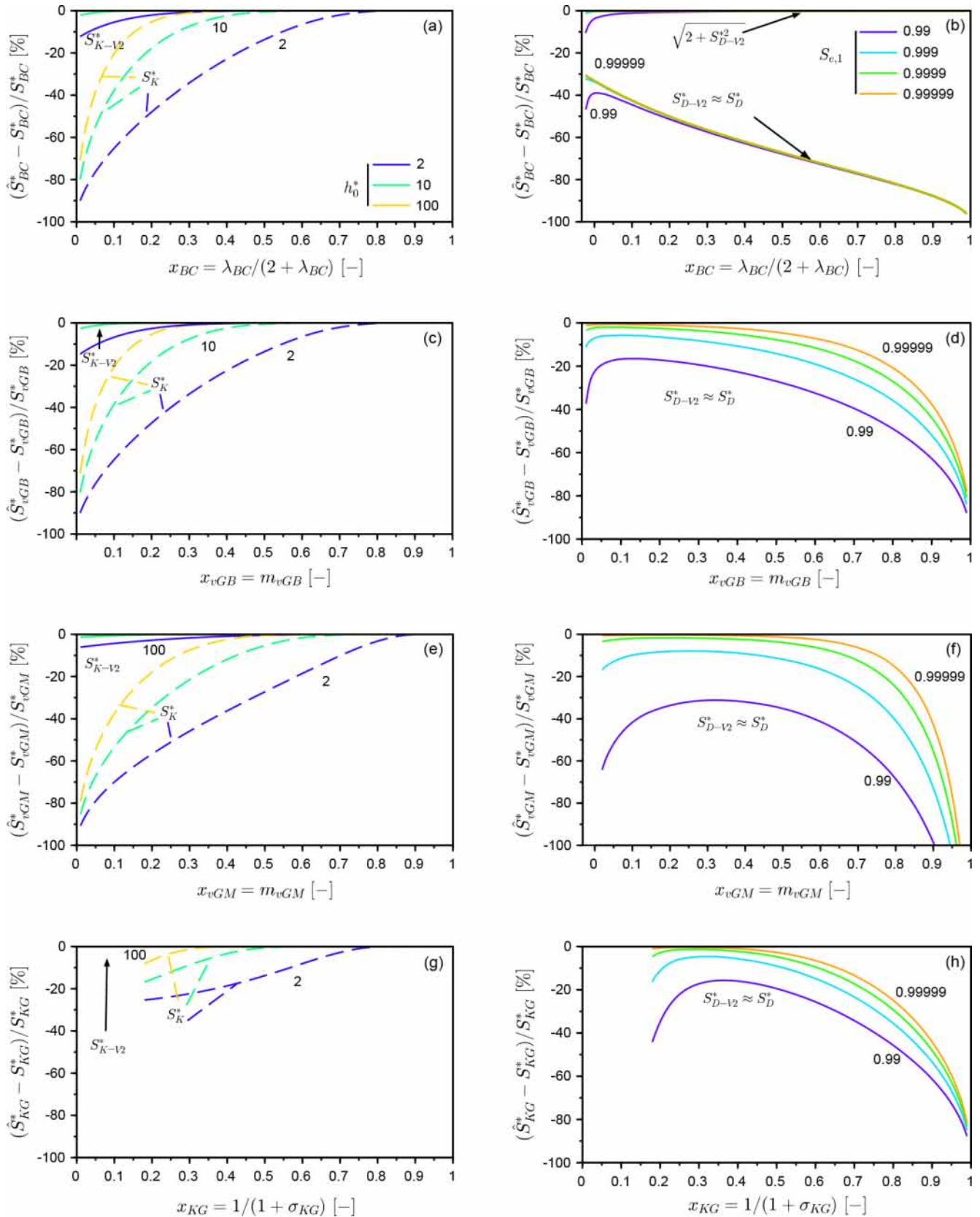
Figure 6. Relative errors of estimators S_D^* and S_{D-v2}^* ( b, d, f, h ) and S_K^* and S_{K-v2}^* ( a, c, e, g ) for the four selected hydraulic models, i.e., BC, vGB, vGM, and KG models, as a function of the WR shape indices.
