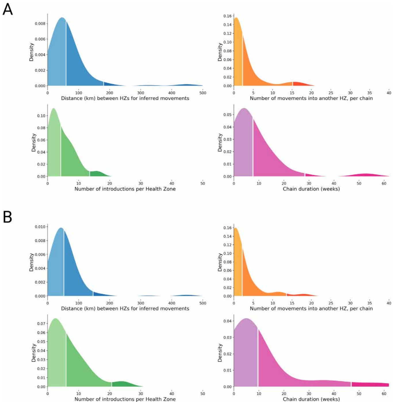
Extended Data Fig. 3 | Inferred transmission dynamics are robust to sampling. a , Kernel density estimates for the same metrics presented in Fig. 3. This analysis used a dataset subsampled to include 3 genomes per health zone per month (total n = 323 genomes). b , Kernel density estimates for the same metrics presented in Fig. 3. This analysis used a dataset subsampled to include 5 genomes per health zone per month (total n = 433 genomes). Inferences from the subsampled datasets recapitulate the findings shown in Fig. 3, suggesting that phylogeographic inferences are robust to sampling frame.
