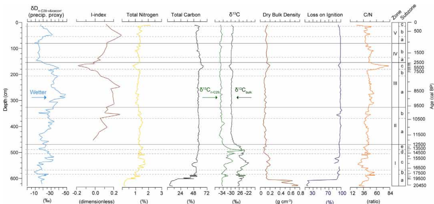
Fig. 8. Proxies of CEN-17.4 including the precipitation proxy ( \delta D_{n-C29-v&icor} (‰), Garcin et al., 2022), I-index (Garcin et al., 2022), total carbon and nitrogen (%), \delta^{13}C_{bulk} (‰) (right, dark green) and \delta^{13}C_{n-C29} (‰) (left, light green, Garcin et al., 2022), dry bulk density ( g\ cm^{-3} ), loss on ignition (%), and C/N ratio plotted against depth (cm) and age (cal BP). Pollen assemblage zones and subzones are also shown.
