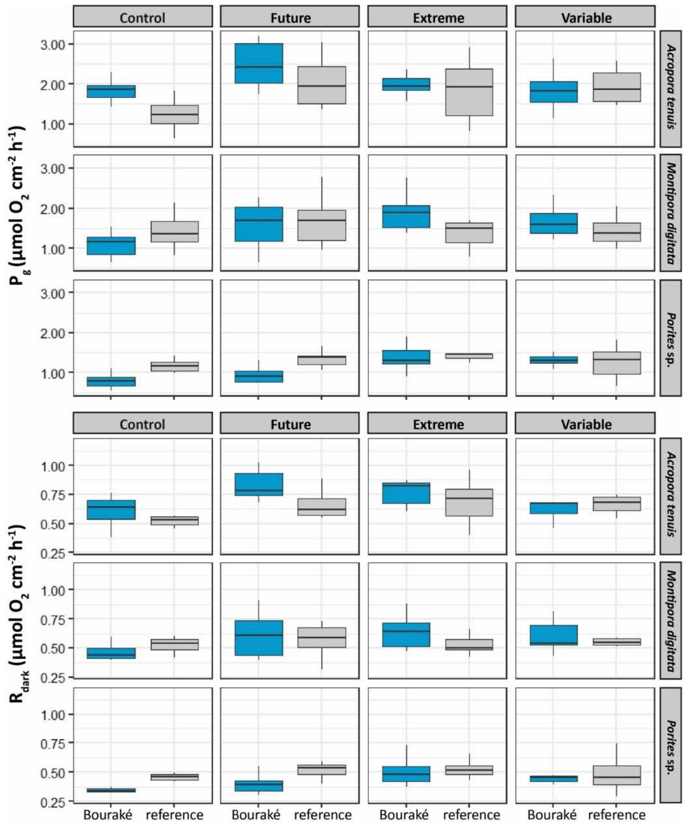
FIGURE 4 Gross photosynthesis ( P_g ) and respiration ( R_{dark} ) rates of corals from Bouraké (in blue) and the reference (in gray) site at four pH conditions (Control, \text{pH}_{\text{NBS}} 8.11; Future, \text{pH}_{\text{NBS}} 7.76; Extreme, \text{pH}_{\text{NBS}} 7.54; and Variable, \text{pH}_{\text{NBS}} 7.56–8.07). Data are median \pm 25th and 75th percentiles ( n = 7 ); see Table S7 for all post hoc comparisons.
