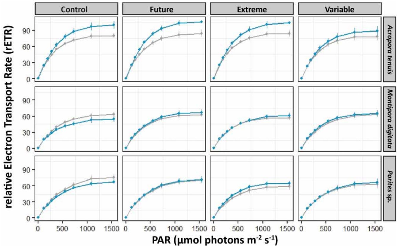
FIGURE 3 Relative electron transport rate (rETR) measured during RLC curves of corals after 100 days of incubation at four pH conditions (Control, \text{pH}_{\text{NBS}} 8.11; Future, \text{pH}_{\text{NBS}} 7.76; Extreme, \text{pH}_{\text{NBS}} 7.54; and Variable, \text{pH}_{\text{NBS}} 7.56–8.07). Bouraké corals are in blue, while reference corals are in gray. Data are mean \pm SE; n = 12 –16, depending on species and pH condition; see Table S7 for all post hoc comparisons.
