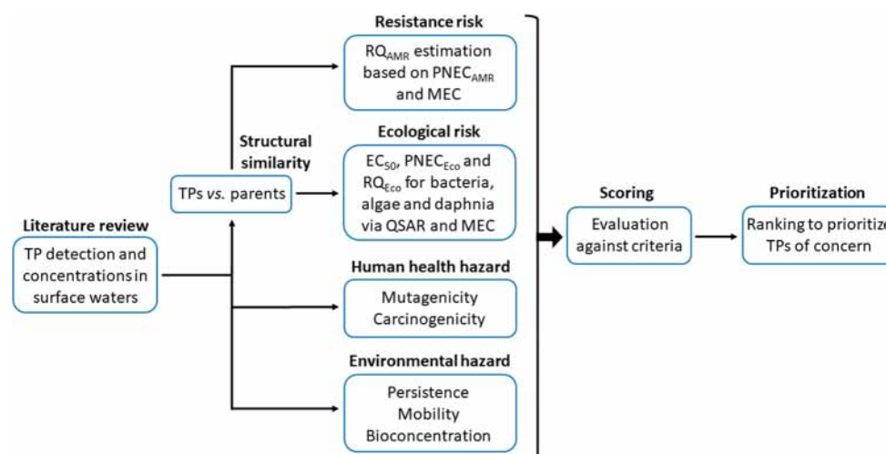
Figure 1. Workflow of meta-analysis in this review to prioritize TPs of concern in surface water environments. RQ_{AMR} : risk quotient of antimicrobial resistance; RQ_{eco} : ecological risk quotient concerning three different species ( RQ_{species} ); PNEC_{AMR} : predicted no-effect concentration for antimicrobial resistance; PNEC_{eco} : predicted no-effect concentration for ecological risk; MEC: measured environmental concentrations; EC_{50} : 50% effect concentration.
