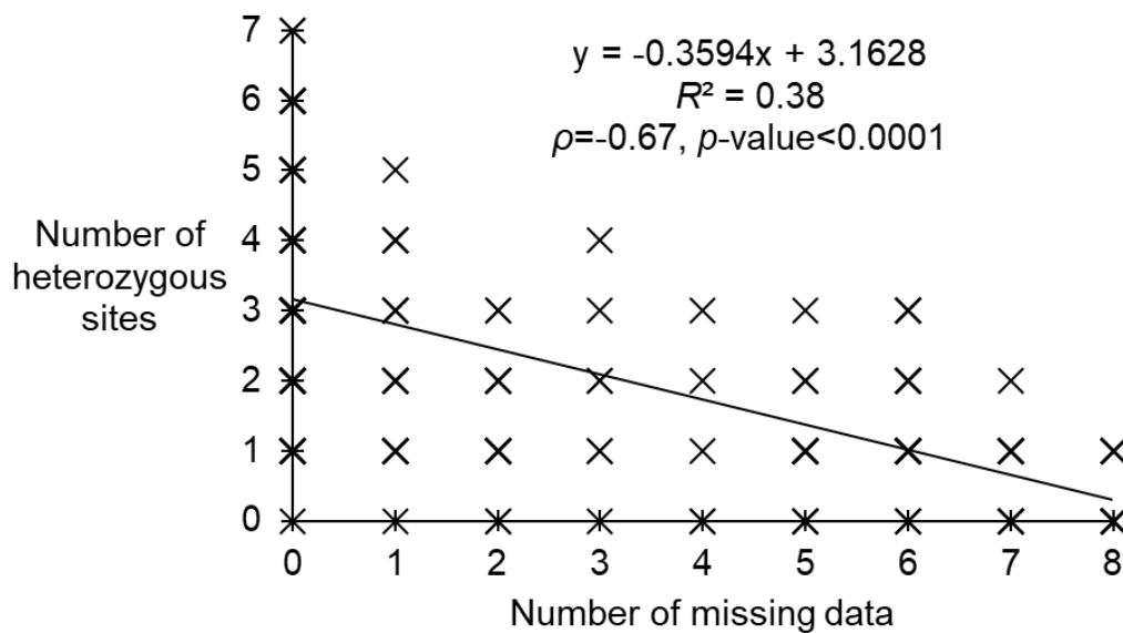
Figure 1: Correlation between the number of missing genotypes (blanks or not interpretable results) and the number of heterozygous sites in Trypanosoma lewisi isolates. Regression equation and determinant coefficient are presented for the sake of illustration. Spearman's rank correlation and one-sided test outputs are also provided
