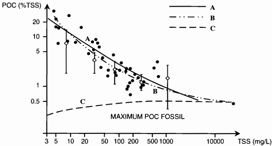
Figure 15.25 Global range of POC (%TSS) and TSS annual averages for major rivers. (For detailed data, see Meybeck, M. and A. Ragu. 1996. River discharges to the oceans: An assessment of suspended solids, major ions, and nutrients. Environment Information and Assessment Rpt. UNEP, Nairobi, 250 pp.). Vertical bars: distribution for given TSS classes from Ittekkot (1988). (a) Initial global regressions of Meybeck (1982). (b) Corrected regression of Meybeck (1993b). (c) Maximum fossil POC hypothesis of Meybeck (1993b).
