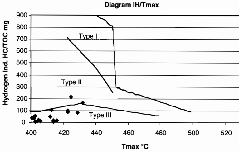
Figure 19.3 HI as a function of Tmax and organic matter type.
