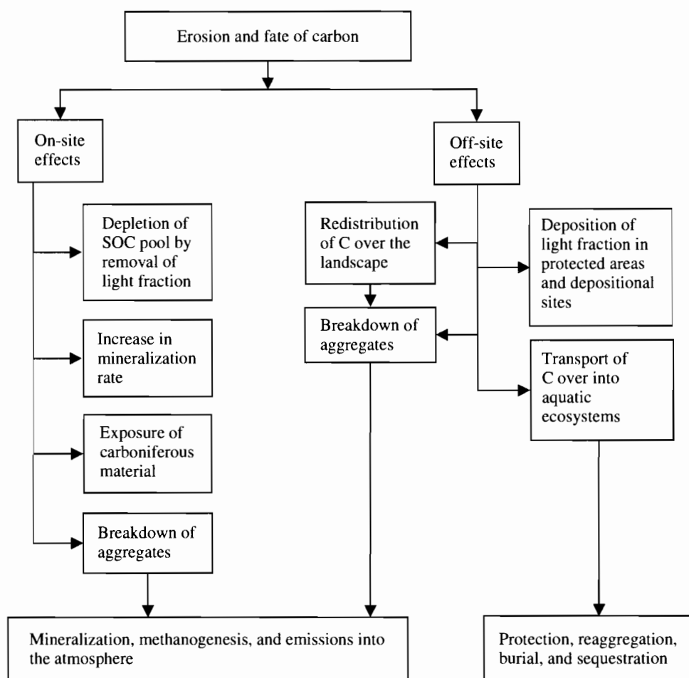
Figure 3.1 Soil carbon dynamics in relation to the accelerated soil erosion by water and wind.
