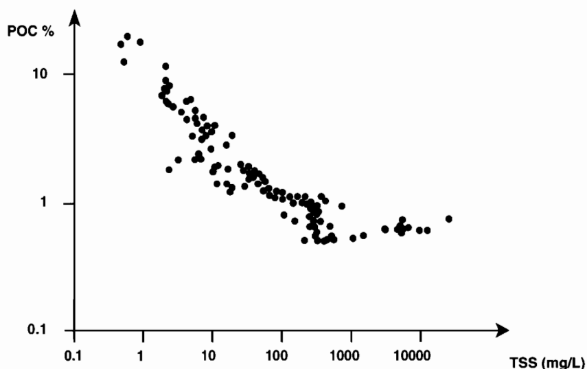
Figure 15.17 Relation between POC contents in suspended matter (%TSS) and TSS in the Lanyang-Hsi River, Taiwan. Note the stabilized POC% above 1000 mg TSS/L. (Data from Kao, S. J. and K. K. Liu, 1997. Fluxes of dissolved and nonfossil organic particulate organic carbon from a small Oceania river (Lanyang Hsi) in Taiwan. Biochemistry 39:255, 269.)
