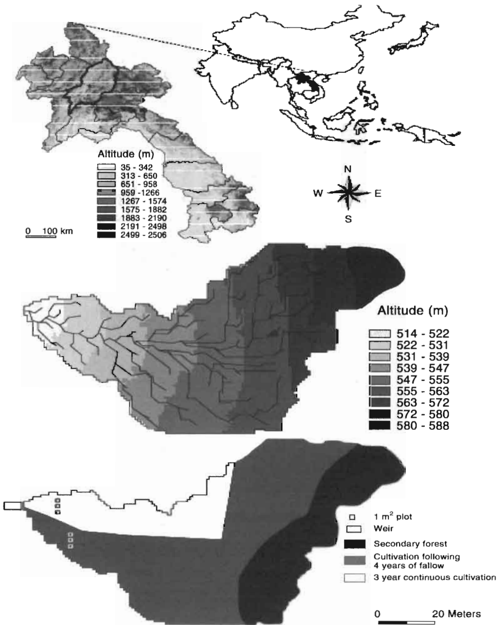
Figure 12.1 Location of the study catchment within the Luang Prabang province (Laos). Topographic conditions and estimated flow pathways from the digital elevation model with a 5-m mesh. Land-use type and history and position of micro-plots for the evaluation of runoff, sediment, and carbon losses.
