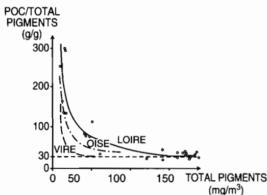
Figure 15.13 Relation between the POC/total pigments ratio (g/g) vs. total pigments in the Loire River compared to two other eutrophied French rivers: Oise (Seine tributary) and Vire (Normandy). (Data from Dessery, S., C. Dulac, J. M. Laurenceau, and M. Meybeck. 1984. Archiv. für Hydrobiol. 100, 2:235–260; Meybeck, M., G. Cauwet, S. Dessery, M. Somville, D. Gouleau, and G. Billen. 1988. Estuarine Coastal Shelf Sci. 27:595–624.)
