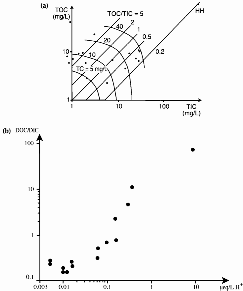
Figure 15.2 Organic carbon vs. inorganic carbon in world rivers. (a) Total organic carbon (TOC) vs. total inorganic carbon (TIC) (Data from Meybeck, M. and A. Ragu. 1996. Environment Information and Assessment Rpt. UNEP, Nairobi, 250 pp.) Diagonal lines represent the equal TOC/TIC ratios and curves the total carbon ( TC = TOC + TIC ). Note the specific position of the Huang He (HH). (b) DOC/DIC ratio vs. proton concentrations ( \mu\text{eq/L} ) in some world rivers, annual averages (Data set from Meybeck, M. and A. Ragu. 1996. Environment Information and Assessment Rpt. UNEP, Nairobi, 250 pp.; and others.)
