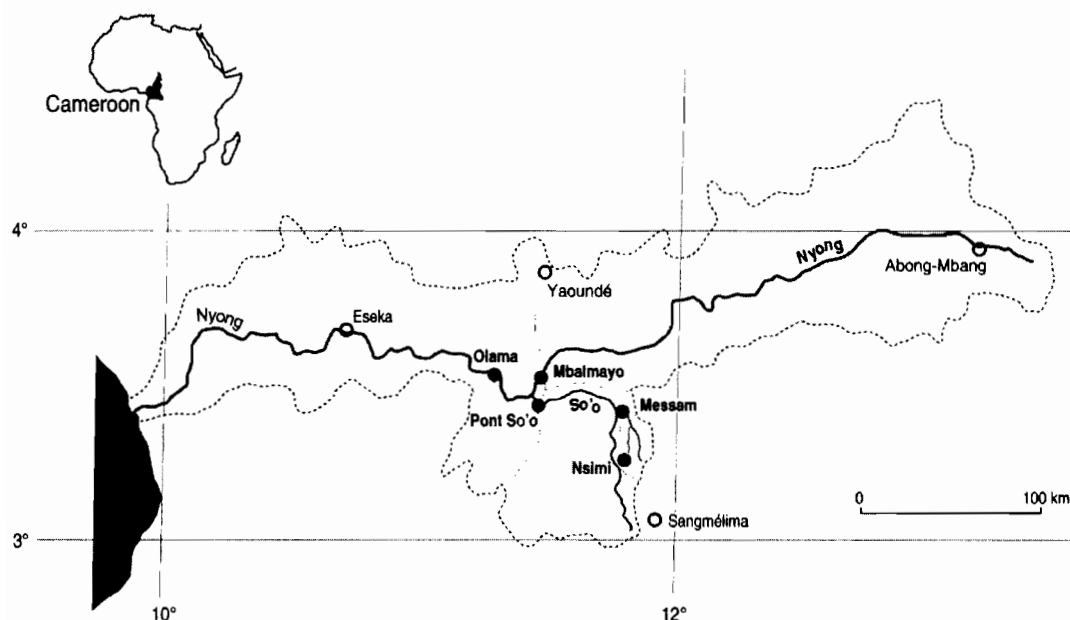
Figure 18.1 Location map of the Nyong basin (southern Cameroon); the studied stations are indicated by black circles.
