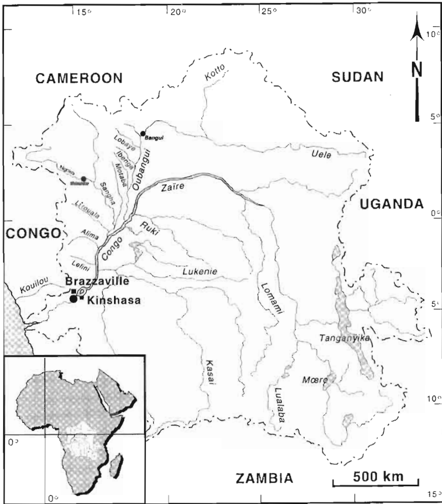
Figure 17.1 Map of the Congo-Zaire basin showing the location of collection sites.
