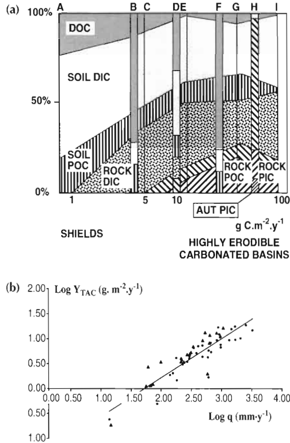
Figure 15.24 Exportation of total carbon by rivers. (a) Decomposition of carbon species exportation in a gradient of total carbon (TC) exportation gCm -2 y -1 . A = Gambia, B = Zaire, C = Mississippi, D = Solimoes, E = Chiang Jiang, F = Negro, G = Brahmaputra, H = Huang He, I = Dranse. (Data from Meybeck, M. 1993a. C, N, P, and S in rivers: From sources to global inputs, in R. Wollast, F. T. Mackenzie, and L. Chou, eds., Interaction of C, N, P and S Biogeochemical Cycles and Global Change . Springer-Verlag, pp. 163–193.) (b) Yield of riverine total atmospheric carbon (g C m -2 yr -1 ) vs. runoff (mm yr -1 ) for major rivers. (Data from Meybeck and Ragu 1996, triangles: highly carbonated basins, log-log scale.)
