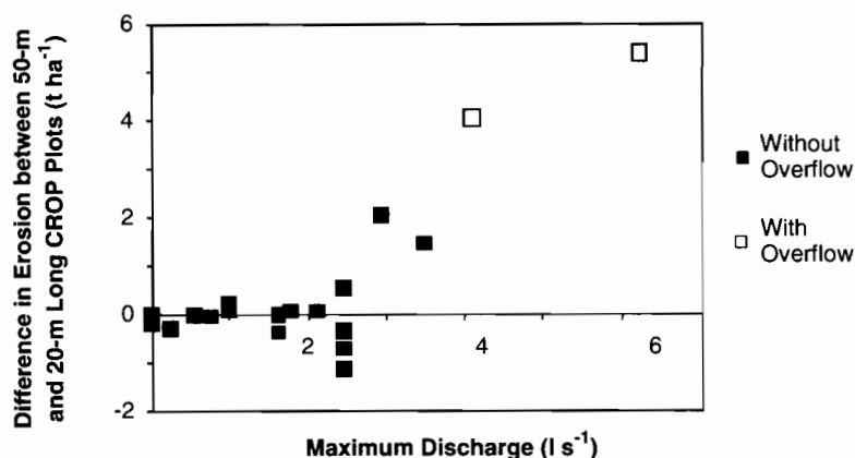
Figure 9.3 Difference in erosion between 50-m- and 20-m-long CROP plots, in relation to maximal discharge on the 50-m-long plot.
