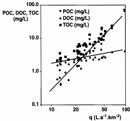
Figure 15.9 Dissolved (DOC), particulate (POC), and total (TOC) organic carbon concentrations on individual samples (mg/L) in the Rhone River at mouth vs. specific discharge q during an exceptional wet year (log scales). (Data from Sempere, R., B. Charriere, F. van Wambeke, and G. Cauwet. 2000. Carbon inputs of the Rhône River to the Mediterranean Sea: Biochemical implications. Global Biogeochem Cycles 14:669–681.)
