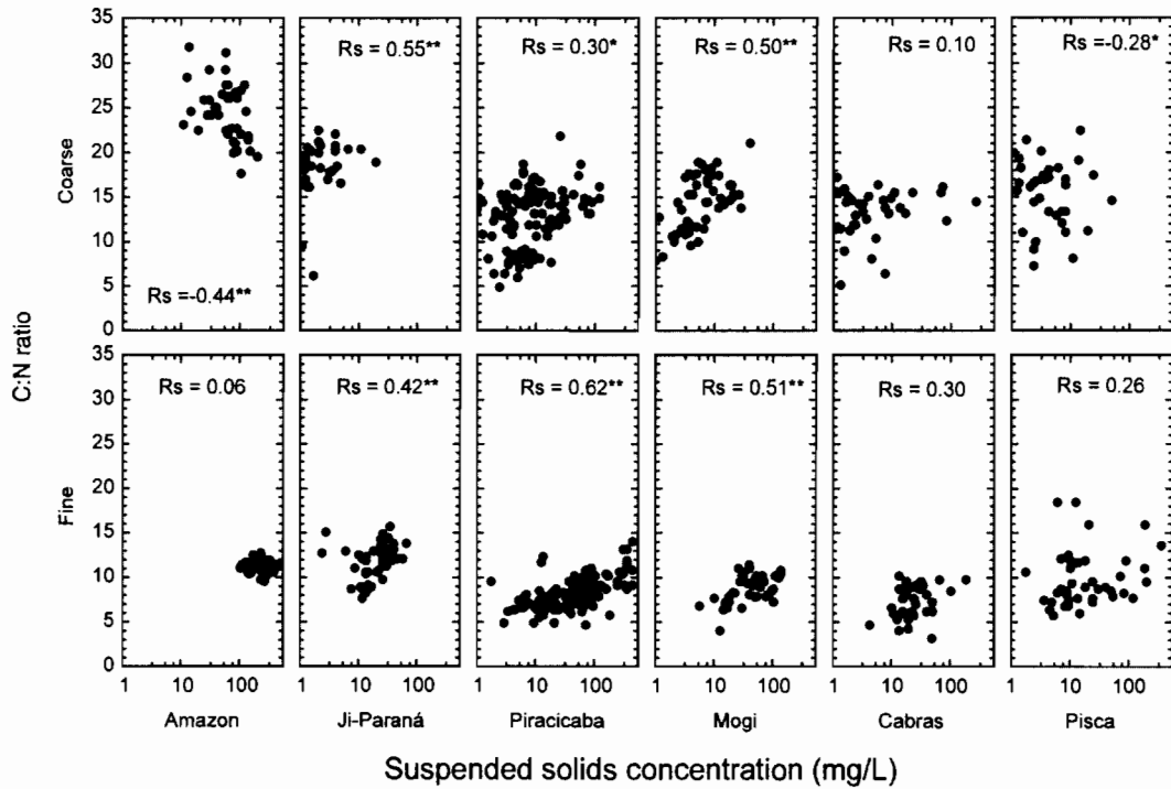
Figure 16.5 Plot of C:N vs. suspended solids concentrations for the coarse and fine size fractions in the Amazon, Ji-Paraná, Piracicaba, Mogi, Cabras, and Pisca river watersheds.
