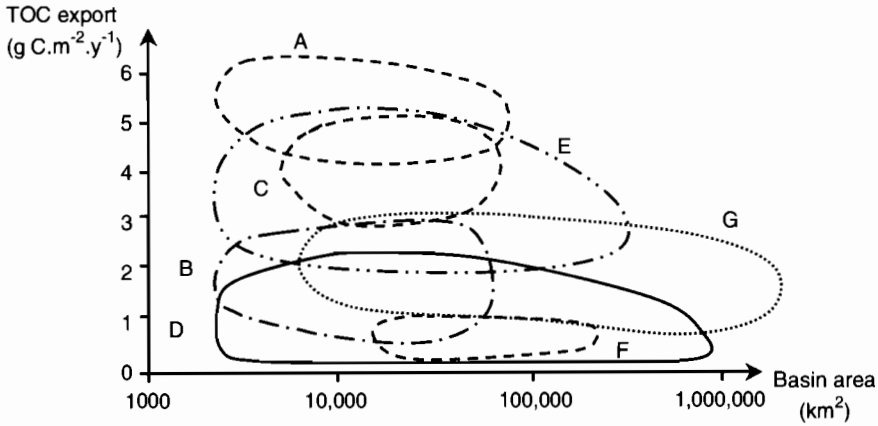
Figure 15.19 Distribution of TOC exportation rates ( \text{g C m}^{-2} \text{yr}^{-1} ) vs. river basin area in six North American regions. A = New Brunswick to Maryland ( n = 13 ), B = Maryland to Georgia ( n = 13 ), C = Florida to Louisiana ( n = 8 ), D = Texas and California to Oregon ( n = 14 ), E = Washington and Alaska ( n = 7 ), F = NW Territories — Nelson Basin ( n = 4 ). (Data from Mulholland, P. J. and J. A. Watts. 1982. Transport of organic carbon to the oceans by rivers of North America: A synthesis of existing data. Tellus 34:176–186.)
