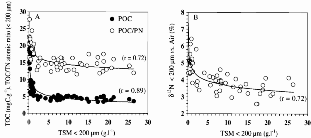
Figure 20.13 Plots of: (a) TOC and TOC/TN vs. TSM and B) d15N vs. TSM for fine-size (< 200 μm) suspended fractions during the June 14, 1998 flood event of the Rio Burate (Boconó watershed, Venezuela). TSM = total suspended matter concentration.
