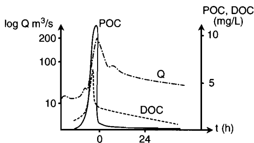
Figure 15.5 Evolution of dissolved (DOC) and particulate (POC) organic carbon concentration during an exceptional flood event in the Cannone mountainstream (Corsica), Mediterranean river regime. (Data from Löye-Pilot, M. D. 1985. Les variations des teneurs en carbone organique (dissous et particulaire) d'un torrent de montagne: La Solenzana, Corse. Verh. Internat. Verein. Limnol. 22:2087–2093. With permission.)
