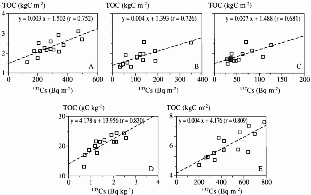
Figure 20.3 Plots of TOC (< 200 μm) vs. 137 Cs inventories of 15 cultivated soils of the Houay Pano catchment (Laos) for several soil depths (a) 0 to 10 cm, (b) 10 to 20 cm, (c) 20 to 30 cm, (d) and (e) integrated 0 to 30 cm. Regression coefficients are displayed between brackets for each plot.
