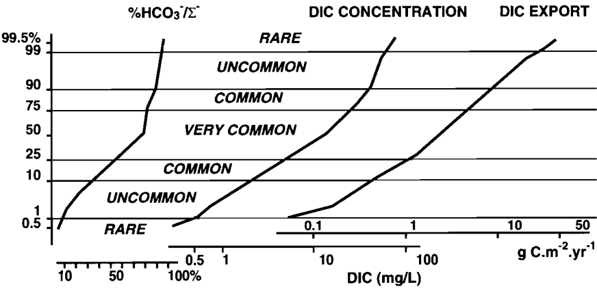
Figure 15.22 Global distribution of DIC concentrations, ionic ratios ( \text{HCO}_3^-/\text{total anions} ), and DIC yields in medium-size pristine basins (vertical scales: probability scale). (From Meybeck, M. 2003b. Global occurrence of major elements in rivers, in K. K. Turekian and H. D. Holland, eds., Treatise of Geochemistry , vol. 5. J. I. Drever, Elsevier, pp. 207–224. With permission.)
