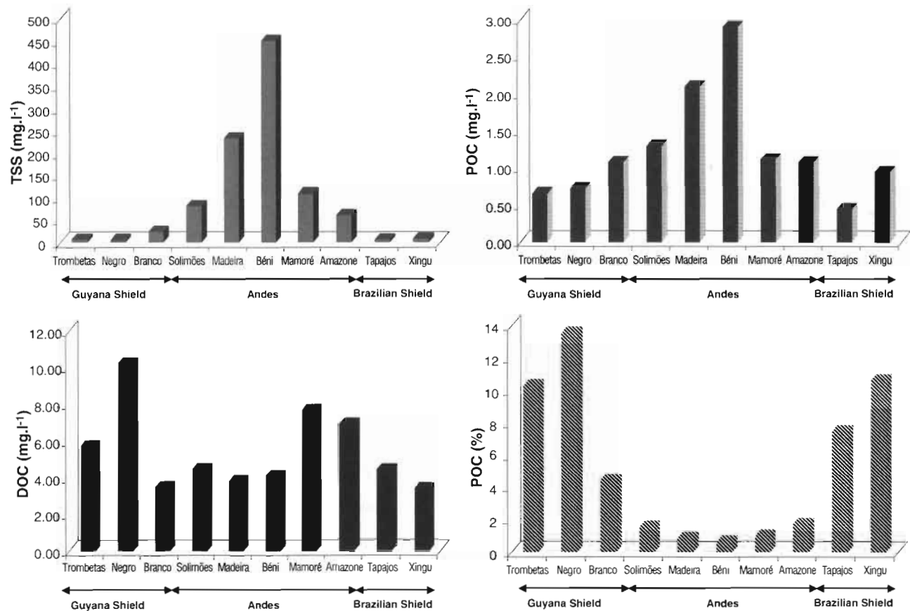
Figure 17.3 Average values of TSS, POC (mg l -1 ), POC%, and DOC in the Amazon basin and its main tributaries.
