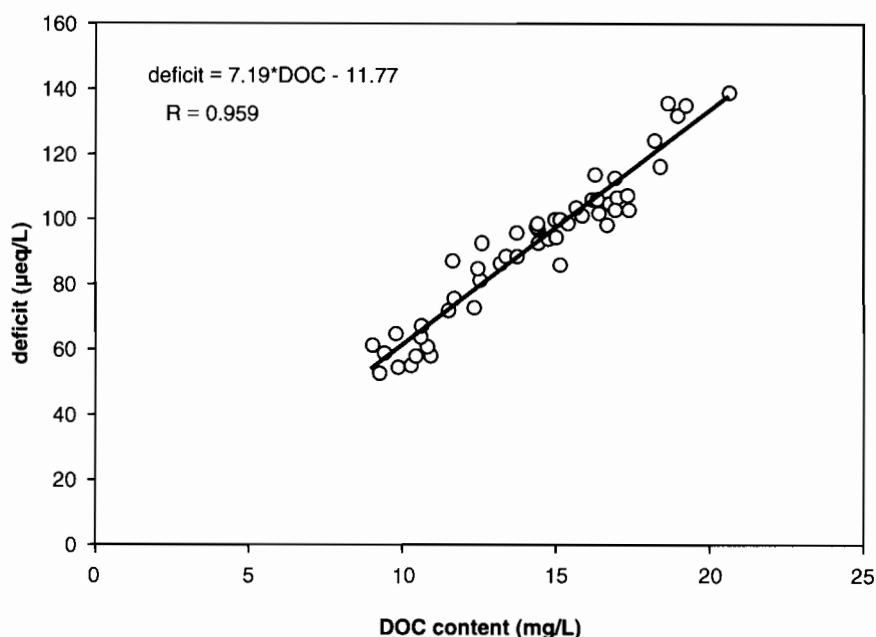
Figure 18.2 Relationship between the anionic deficit and the DOC content in the Mengong River during the year 1998/99.
