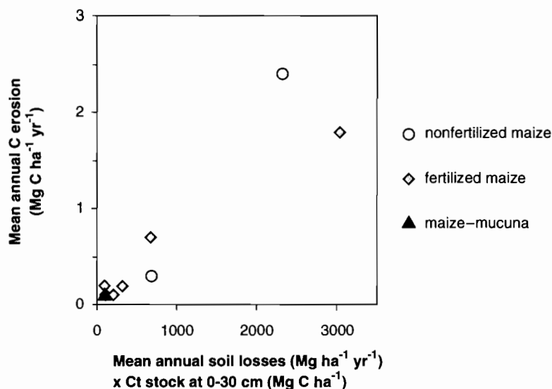
Figure 10.1 Relationship between mean annual C erosion (Mg C ha -1 yr -1 ) and the product of mean annual soil losses (Mg ha -1 yr -1 ) into Ct stock of bulk soil at 0 to 30 cm (Mg C ha -1 ) (data from Table 10.5).
