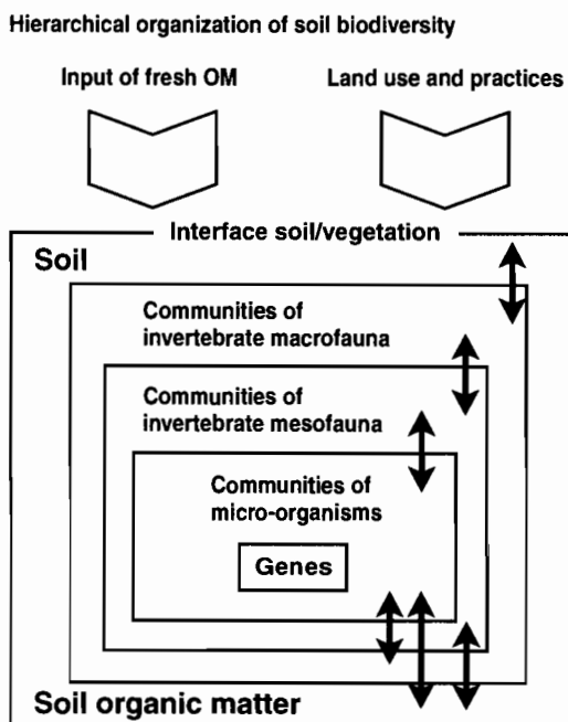
Figure 1.8 Role of soil organic matter in biodiversity. (From Robert, M. 2001. Soil carbon sequestration for improved land management. World Soil Resources Report 96 . FAO, Rome, 57 p. French and Spanish versions, 2002.)
