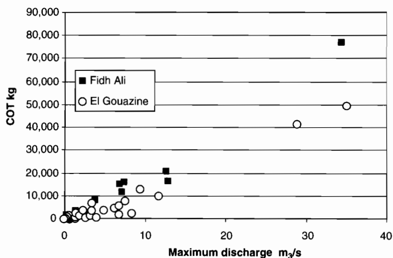
Figure 19.4 TOC flux as a function of peak flow (all are measured data points).
