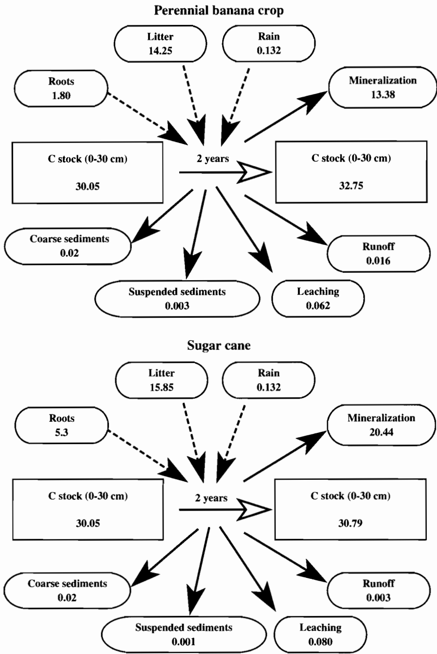
Figure 7.1 C budget in banana and sugarcane treatments (10% slope) showing C stock changes in 2 years (equivalent mass basis) (in \text{Mg C ha}^{-1} ), C inputs (litter, root, and rain) and C outputs (erosion, leaching, and mineralization) (in \text{Mg C ha}^{-1} \text{ 2 yr}^{-1} ).
