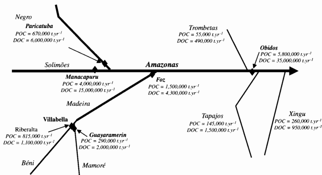
Figure 17.8 Fluvial budget of DOC and POC in the Amazon basin.
