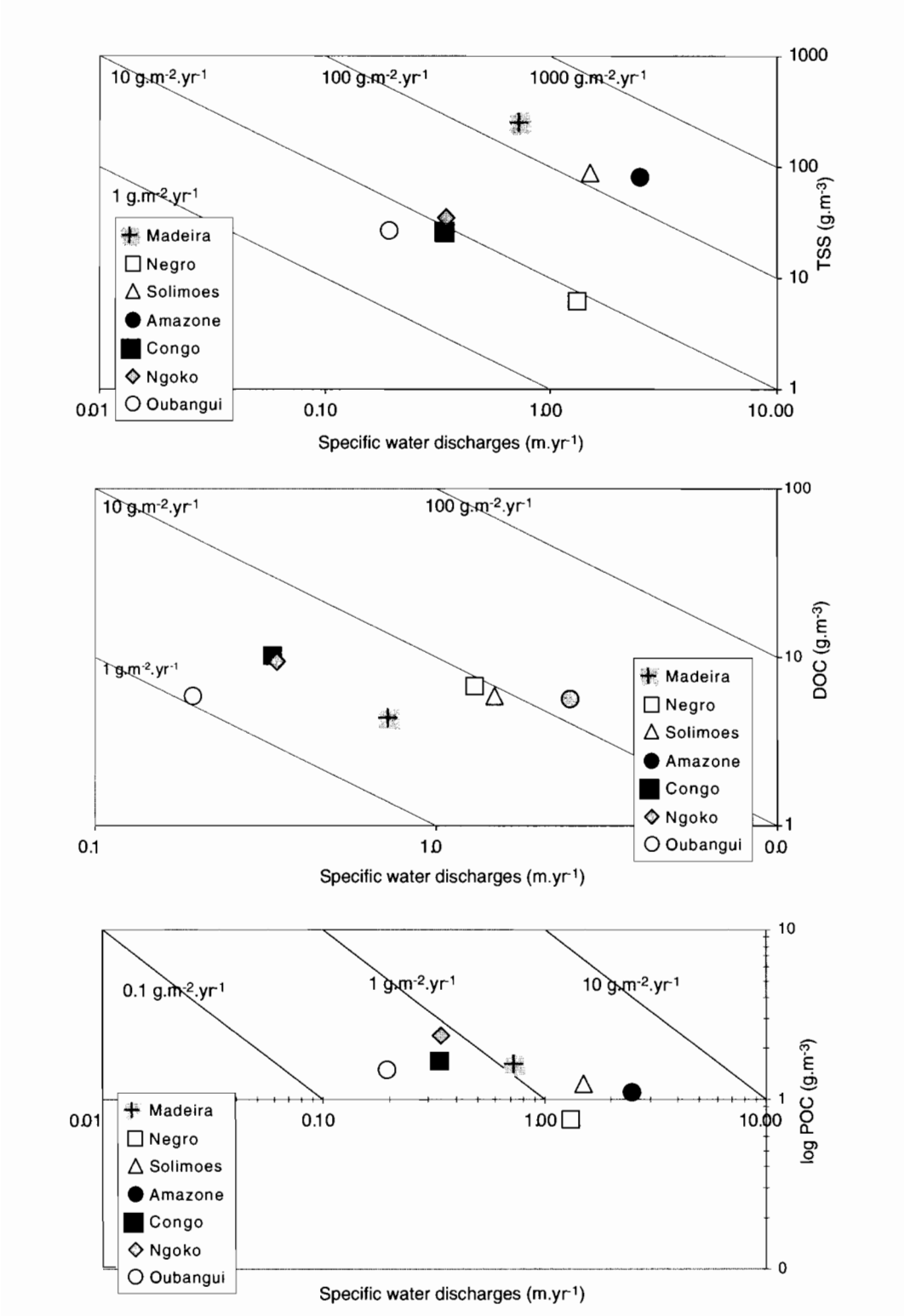
Figure 17.9 Annual specific rates of TSS, POC, and DOC in Congo-Zaire and Amazon basins ( \text{g}\cdot\text{m}^{-2}\cdot\text{yr}^{-1} ).
