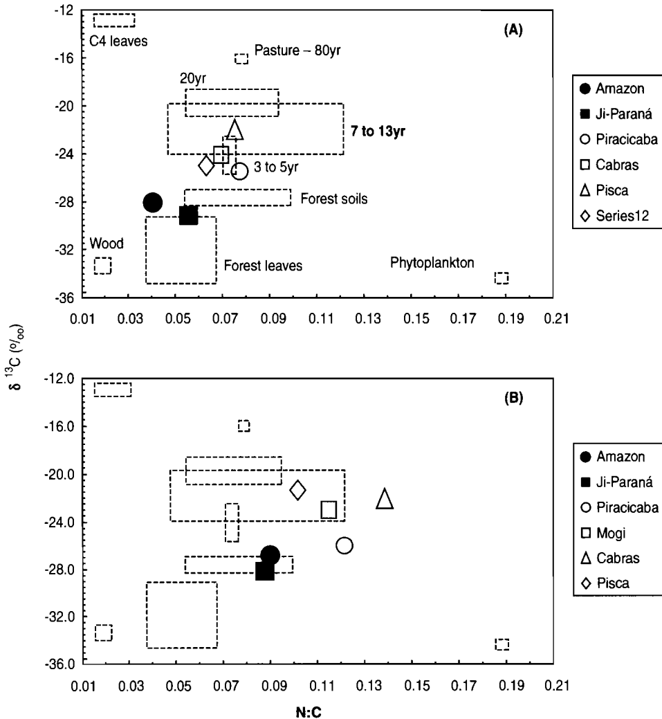
Figure 16.7 Plot of N:C ratio vs. \delta^{13}\text{C} for the coarse (A) and fine (B) size fractions and the following end-members: tree leaves from forests, forest soil, soil covered with a pastures of age between 3 to 5 years, 7 to 13 years, 20 years, and 80 years (rectangles representing the distribution of all points). Tree leaves collected in Ji-Paraná (Martinelli, L. A. and Ehleringer, J. E., unpublished data); forest soil organic matter — soils collected in forests near Manaus and Santarém (Telles, E. V., unpublished data); pasture soils — soils samples collected at several sites in the Rondônia State (Neill et al., 1997).
