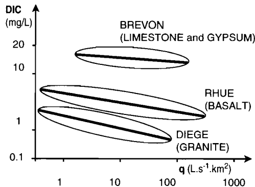
Figure 15.4 Compared evolution of DIC with river runoff in three small monolithic French streams: Brevon (Haute Savoie), Rhue at Egliseeneuve (Auvergne), and Diège (Corrèze).
