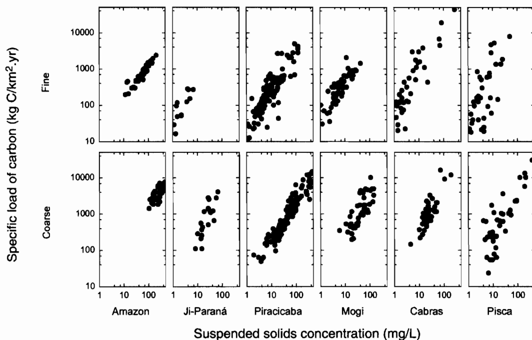
Figure 16.2 Plot of specific load of carbon vs. suspended solids concentrations for the coarse and fine size fractions in the Amazon, Ji-Paraná, Piracicaba, Mogi, Cabras, and Pisca river watersheds.
