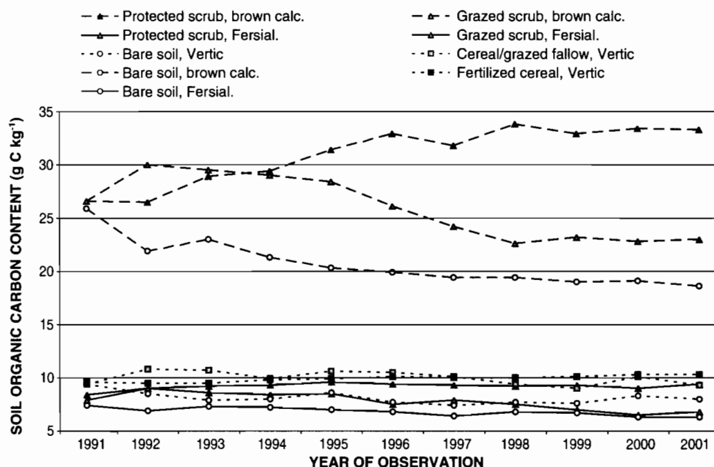
Figure 8.1 Changes in soil organic carbon content at 0 to 10 cm depth in the runoff plots located near Tlemcen (1991 to 2001).
