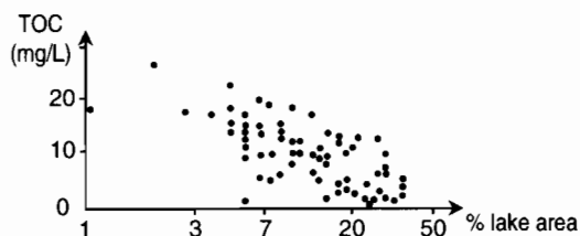
Figure 15.7 Inverse relationship between average TOC concentration and the proportion of lake area in a set of 78 small Finnish basins. (Redrawn from Kortelainen, P. and J. Mannio, 1988. Natural and anthropogenic acidity sources for Finnish lakes. Water Air Soil Poll. 42:341–352.)
