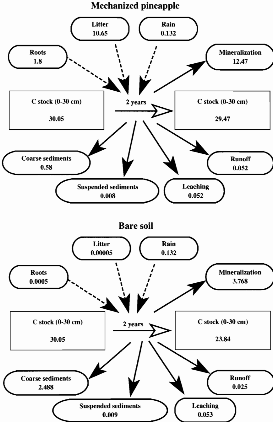
Figure 7.2 C budget in intensive-till pineapple and bare soil treatments (10% slope) showing C stock changes in 2 years (equivalent mass basis) (in Mg C ha -1 ), C inputs (litter, root, and rain) and C outputs (erosion, leaching, and mineralization) (in Mg C ha -1 2 yr -1 ).
