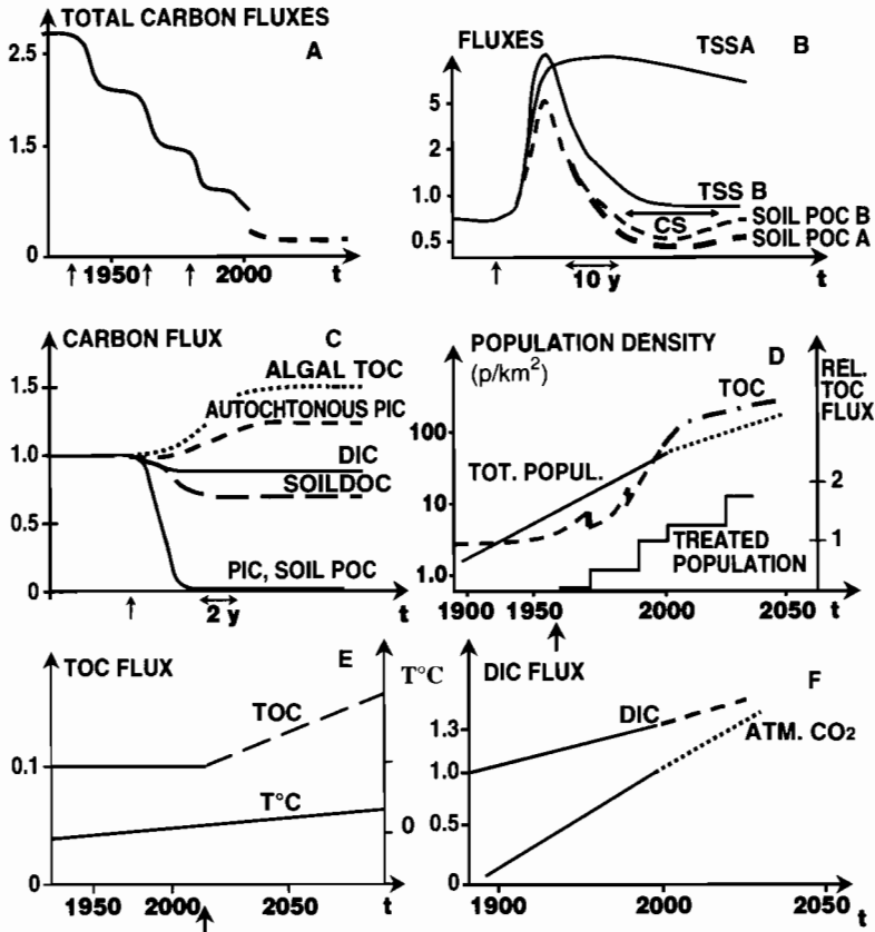
Figure 15.28 Working hypotheses for the contrasted future of carbon fluxes at the Anthropocene. (All fluxes are normalized to pristine average conditions.) (a) Stepwise reduction of fluxes in near-arctic rivers with water consumption periods. (b) Stepwise evolution of TSS and soil POC, without proper soil conservation practices (1) and with soil recovery (2); (CS = soil organic carbon sequestration). (c) Contrast trends after damming (settling vs. autochthonous carbon production). (d) Nonlinear response of river TOC flux downstream of fast-growing megacity with marked time-lag between population growth and urban sewage collection. (e) Threshold TOC increase due to permafrost melt in arctic basins. (f) Gradual DIC increase in forested area due to CO 2 elevation. (Arrows indicate start of pressure.)
