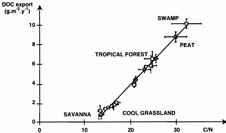
Figure 15.20 DOC export vs. average C/N ratio ( \text{g g}^{-1} ) in contrasted river basins. (From Aitkenhead, J. A. and W. H. MacDowell. 2000. Soil C:N ratio as a predictor of annual riverine DOC flux at local and global scales. Global Biogeochemical Cycles . 14:127–138. With permission.)
