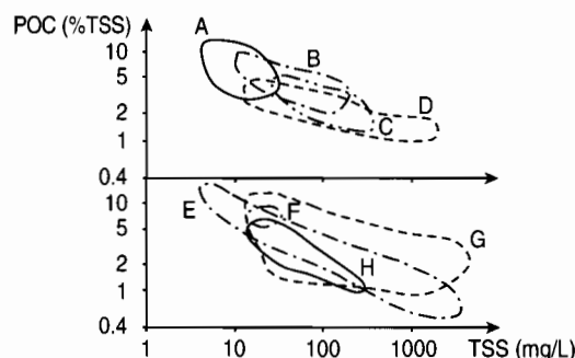
Figure 15.11 Relationship between individual measurements of particulate organic carbon content (POC in %TSS) and total suspended solids (TSS in mg/L): range during one hydrological year. A = Saint Lawrence, B = Niger, C = Mississippi, D = Indus, E = Missouri, F = Zaire, G = Yang Tse, H = Orenoco. (Data from the SCOPE carbon program [Degens et al., 1982] and Mitt. Geol. Pal. Inst. Univ. Hamburg , 52, 55, 58, and 64.)
