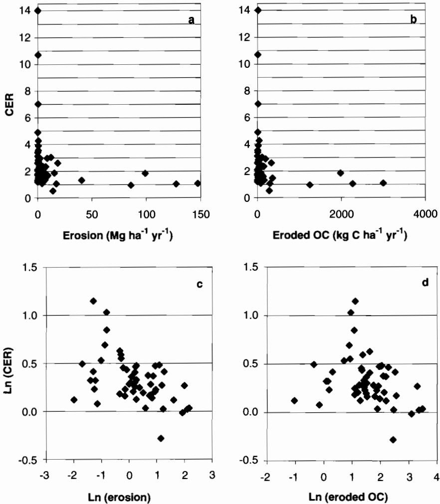
Figure 5.1 Relations between carbon enrichment ratio of sediments (CER) and erosion or eroded OC on the 54 runoff plots under study.
