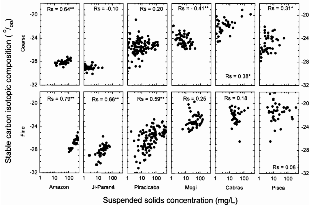
Figure 16.6 Plot of stable carbon isotopic composition ( \delta^{13}C ) vs. suspended solids concentrations for the coarse and fine size fractions in the Amazon, Ji-Paraná, Piracicaba, Mogi, Cabras, and Pisca river watersheds.
