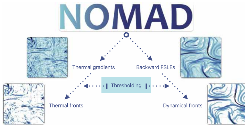
Fig. 1 Illustration showing how NOMAD 51 users can go from thermal gradients (resp. backward FSLEs) to thermal (resp. dynamical) fronts via region-specific thresholding, with example of fields before and after thresholding. All fields were taken on July 1st, 2020. The colormap is from cmocean 80 and with the same range as in Fig. 2.
