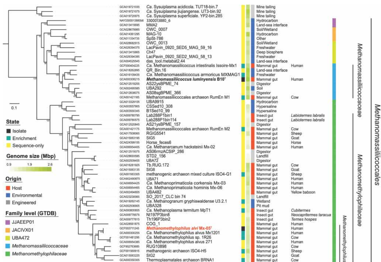
Figure 2. Methanomassiliicoccales maximum likelihood tree built with an LG+F+R10 model from 41 concatenated protein sequences. The tree is rooted on ‘ Candidatus Sysuipasmatales ’ [38], with 10,325 positions after trimming. Values on the tree indicate the bootstrap supports > 70%. The tree was formatted with Itol [45]. Isolated species are indicated in bold.
