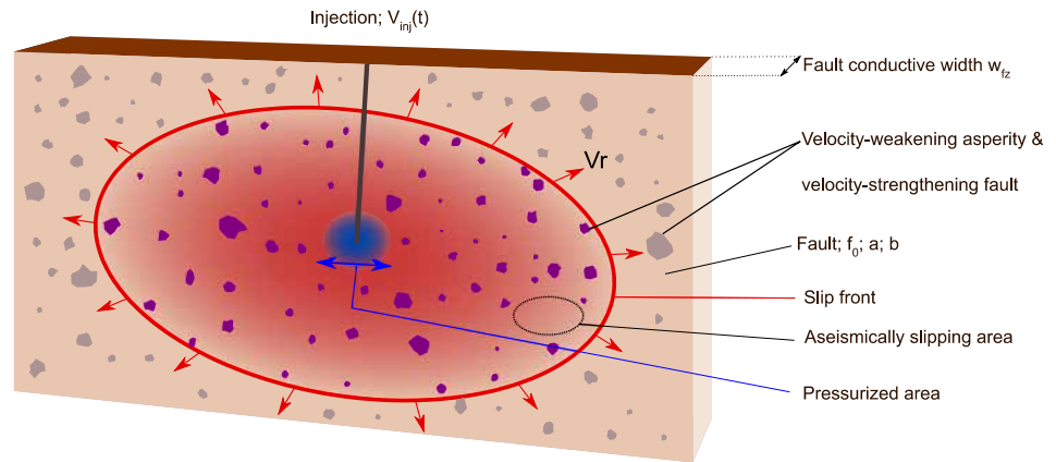
Figure 3. Schematic of the fault model considered. Along a single fault plane of conductive thickness w_{fz} , injection of fluids leads to pressure increase in a small expanding area (blue) which induces an expanding aseismic slip crack of much larger area (red). As the crack propagates, it triggers seismicity on asperities (polygons).
