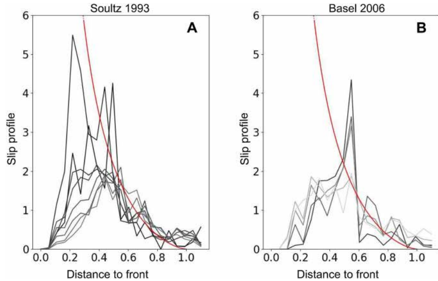
Figure 4. Comparison of the spatial distribution of seismic moment density observed in swarms with aseismic slip predicted by the crack model. The radial distributions for Soultz 1993 (a) and Basel (b) are shown at various times as a function of distance to the origin normalized by the distance to the seismicity front. For each radial bin, the seismic moment density is computed as the sum of the seismic moment of all events with hypocenters lying within the bin, divided by the bin area (a ring). It is then normalized by its average over the area between 0.3 and 1. The curves correspond to the moment computed while injection is occurring (while flow rate is positive) on expanding time windows incremented by 2 days over the first 16 days for Soultz and by 1 day over the first 5 days for Basel (greyscale getting darker with time). The seismicity front position, in this case, is taken as the 95th and 80th percentiles of distance for the non-overlapping 50 events bins considered, for Soultz 1993 and Basel, respectively. The red line represents the theoretical slip profile of the circular crack model loaded by a point pressure (Equation A22), divided by its average slip between normalized distances 0.3 and 1.
