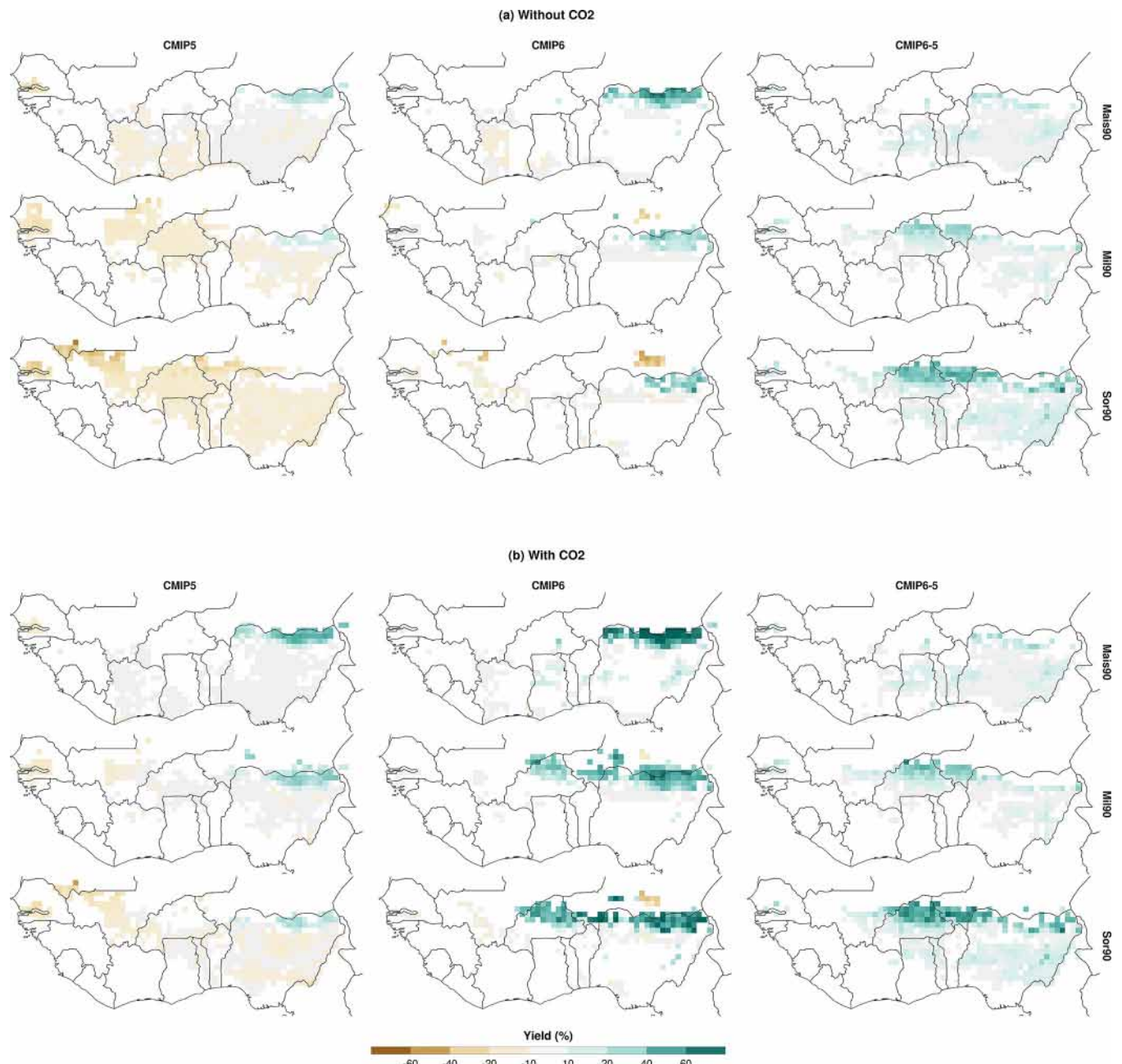
Fig 3. Relative change in mean yields for the varieties of 90 days with and without [CO_2] in West Africa under RCP45/SSP2-4.5 scenario for a near term (2035–2064) as compared with the reference period (1975–2004) in CMIP5, CMIP6 and the difference between CMIP6 and CMIP5 models. Areas with significant changes with 95% confidence level are represented (bootstrap method).
