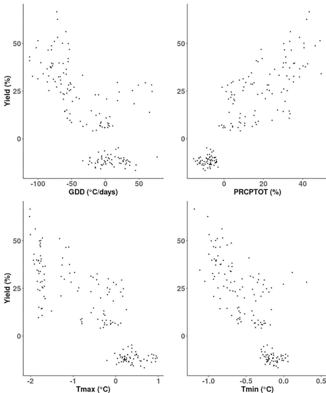
Fig 8. Relationship between climate changes (growing degree days, rainfall, maximum and minimum temperature) and yields changes of sorghum 90-days in the difference between CMIP5 and CMIP6 models. Changes are computed under RCP85/SSP5-8.5 scenario for a long term period (2065–2094) as compared with the reference period (1975–2004). Absolute changes are shown for growing degree days and minimum and maximum temperature, while relative changes were computed for rainfall and crop yields. Positive values indicate higher values of future changes in CMIP6 compared to CMIP5.
