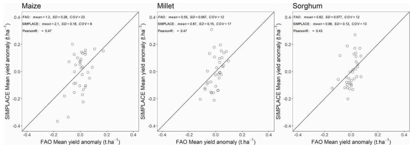
Fig 1. Comparison between simulated crop yield and FAO time series data at the country level for Maize, Millet and Sorghum 5-Year Moving Average. The yields at pixel level were aggregated over West Africa for the estimated period 1979–2013 with MIRCA2000 landuse data using EWEMBI climate dataset. Pearson correlation coefficient (R) was calculated between FAO and Simplace yields.
