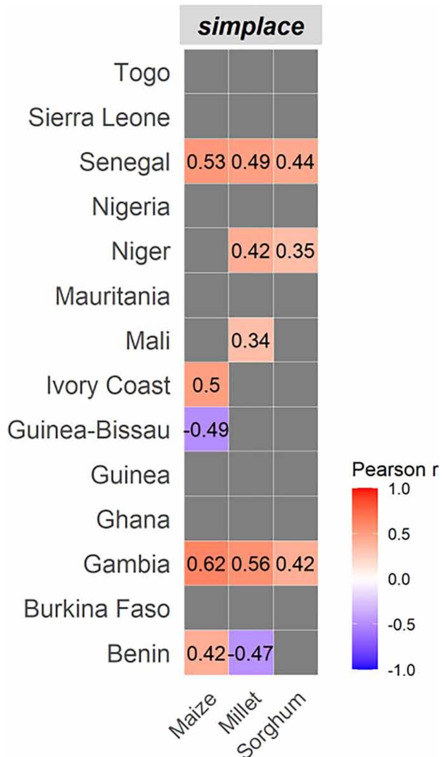
Fig 2. Heatmap of the Pearson correlation coefficient (R) between the simulated and observed FAO country level mean yields for maize, pearl millet and sorghum 5-Year Moving Average. Yields at pixel level were aggregated over countries with MIRCA2000 land use data and Pearson correlation coefficient R calculated over the period 1979–2013. Grey boxes indicate that correlations are not statistically significant (p-value > 0.05).
