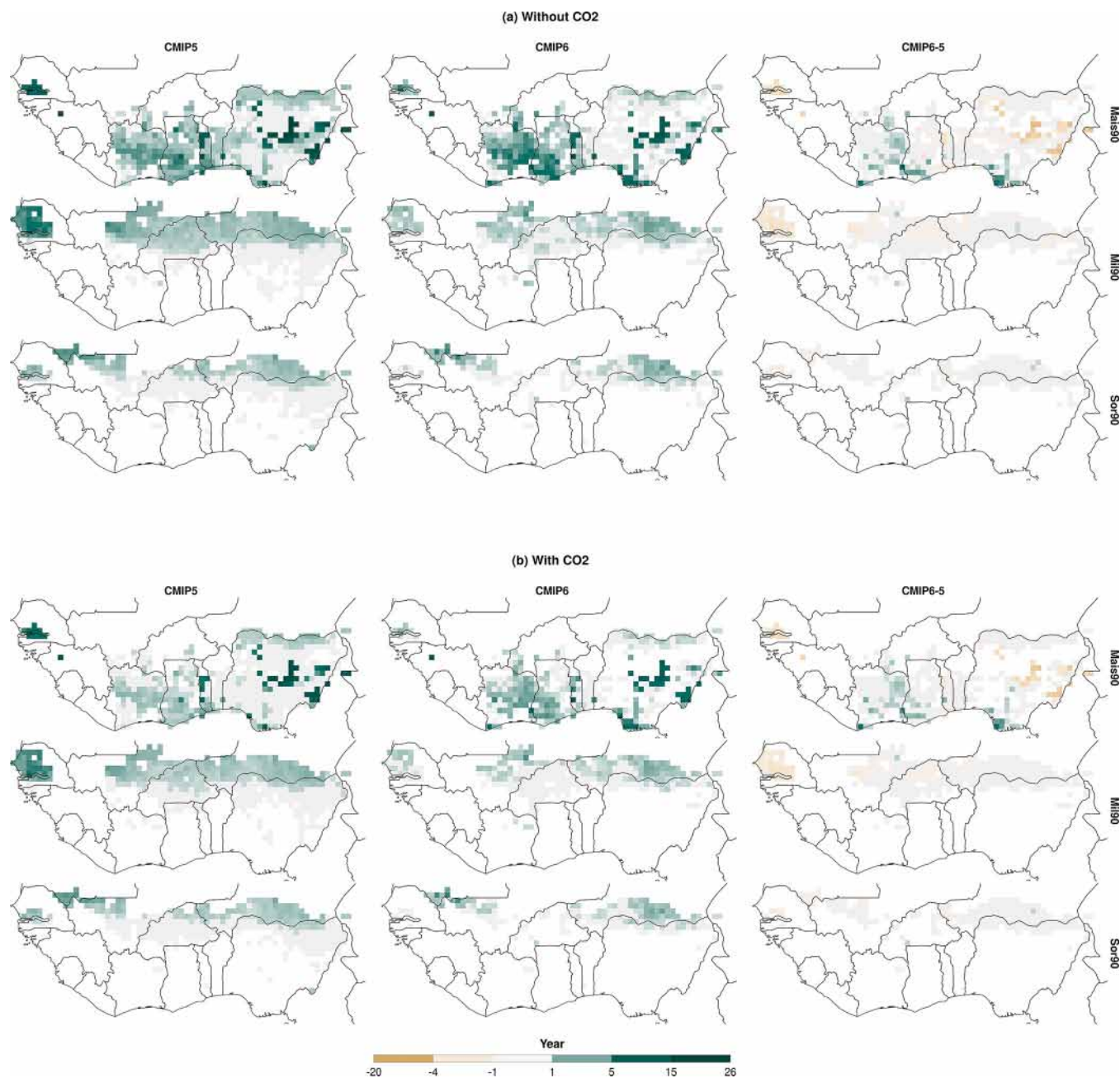
Fig 5. Relative change in the number of years of crop failure for the varieties of 90 days with and without [CO 2 ] in West Africa under RCP45/SSP2-4.5 scenario for a near term (2035–2064) as compared with the reference period (1975–2004) in CMIP5, CMIP6 and the difference between CMIP6 and CMIP5 models. A crop failure is defined as a year with a simulated yield below the 10% quantile of historical yields. Areas with significant changes with 95% confidence level are represented (bootstrap method).
