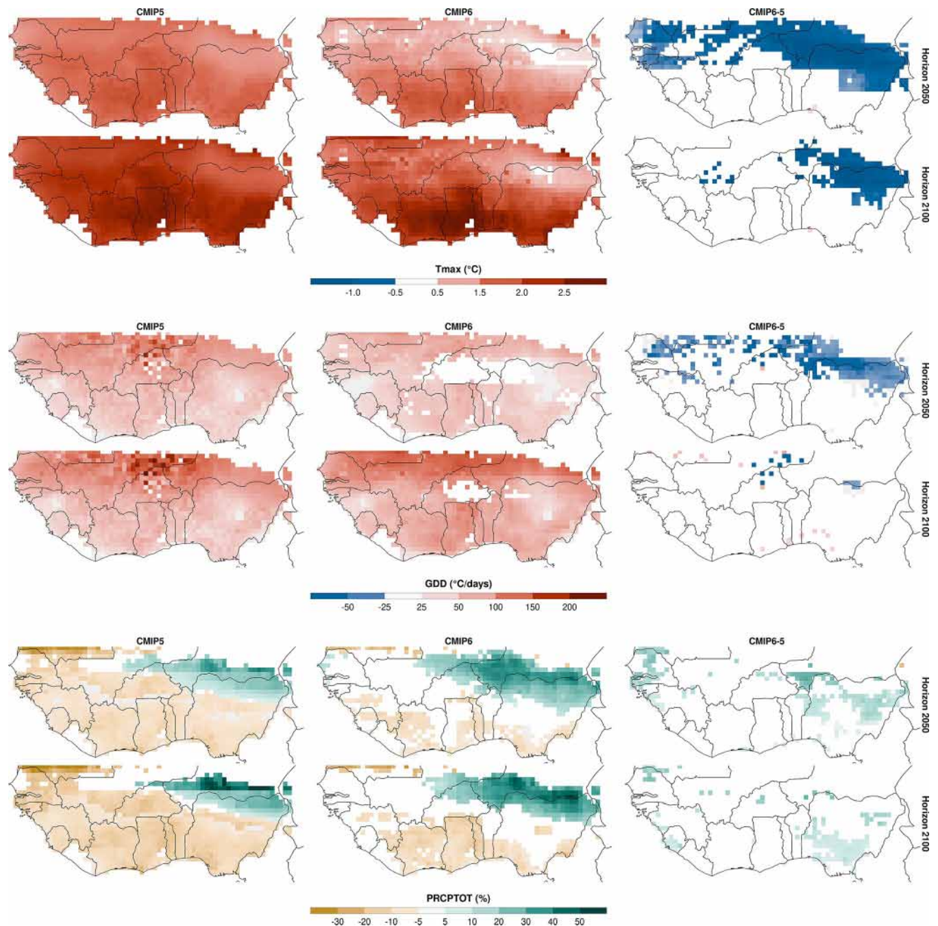
Fig 7. Future changes in maximum temperature ( ^{\circ}\text{C} ), growing degree days ( ^{\circ}\text{C}/\text{days} ) and precipitation (%) over West Africa under RCP45/SSP2-4.5 scenario for the two time periods (2035–2064 and 2065–2094) as compared with the reference period (1975–2004) in CMIP5, CMIP6 and the difference between CMIP6 and CMIP5 models. Areas with significant changes with 95% confidence level are represented (bootstrap method).
