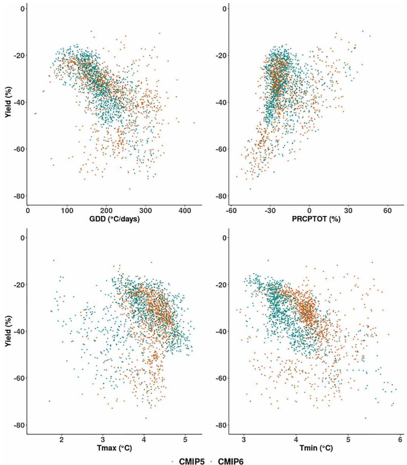
Fig 6. Relationship between climate changes (growing degree days, rainfall, maximum and minimum temperature) and relative change in mean yield of sorghum 90-day in CMIP5 and CMIP6 models. Changes are computed under RCP85/SSP5-8.5 scenario for a long term period (2065–2094) as compared with the reference period (1975–2004). Absolute changes are shown for growing degree days and minimum and maximum temperature, while relative changes were computed for rainfall and crop yields. The orange circles represent future changes projected in CMIP5 and CMIP6 is presented in cyan. This figure has a restricted y axis to zero in relative change in mean yield to enhance the clarity of the results and exclude the most extreme pixels (five pixels over 2250 pixels were excluded).
