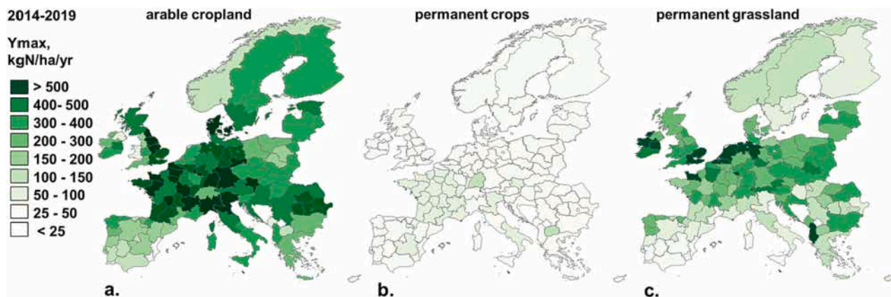
Fig. 4. Regional distribution of Ymax in arable cropland (a), permanent crops (b) and permanent grasslands (c) in Europe, as calibrated from the results of the GRAFS analysis at regional resolution over the period 2014–2019.
